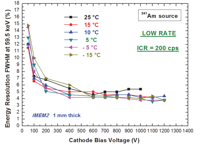
Fig. 5. Energy resolution (FWHM) at 59.5 keV vs. the bias voltage at different temperatures for the IMEM2 detector. The analog electronics with a shaping time constant of 1 \mu\text{s} was used.
