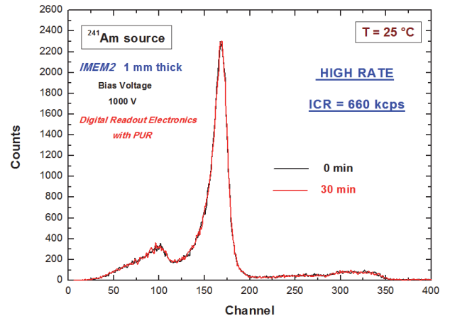
Fig. 9. The measured ^{241}\text{Am} spectra (ICR = 660 kcps) of the IMEM2 detector, just after biasing (black line) and after 30 minutes (red line). The digital electronic with a ST = 5\ \mu\text{s} , equipped with a pile-up rejection (PUR) was used.
