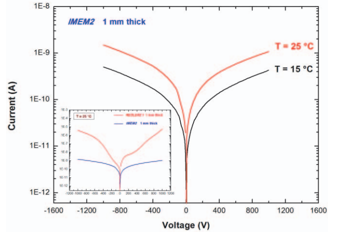
Fig. 2. The current-voltage characteristics of the 1 mm thick CZT detector at (IMEM2) room temperature ( T=25^\circ\text{C} ) and at T = 15^\circ\text{C} . The inset also shows the current-voltage curves of both IMEM2 and REDLEN2.1 (1 mm thick) at room temperature.
