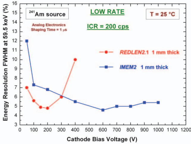
Fig. 6. Energy resolution (FWHM) at 59.5 keV vs. the bias voltage at room temperature for the IMEM2 and REDLEN2.1 detectors. The analog electronics with a shaping time constant of 1\ \mu\text{s} was used.
