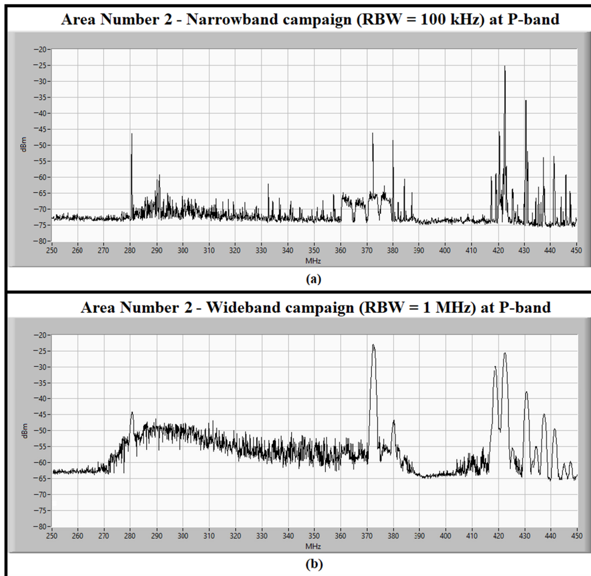
Figure 3. (a) The P-band spectrum, between 250 and 450 MHz, measured in the narrowband campaign (i.e., spectrum analyzer RBW set to 100 kHz) for detection of continuous signals in area number 2; (b) The P-band spectrum, between 250 and 450 MHz, measured in the wideband campaign (i.e., RBW set to 1 MHz) for detection of impulsive signals in area number 2.
