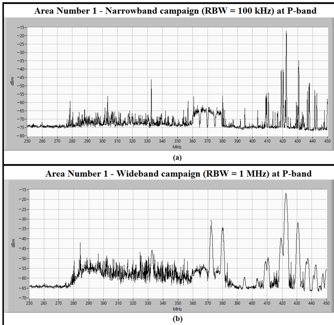
Figure 2. (a) The P-band spectrum, between 250 and 450 MHz, measured in the narrowband campaign (i.e., spectrum analyzer RBW set to 100 kHz) for detection of continuous signals in area number 1; (b) the P-band spectrum, between 250 and 450 MHz, measured in the wideband campaign (i.e., RBW set to 1 MHz) for detection of impulsive signals in area number 1.
