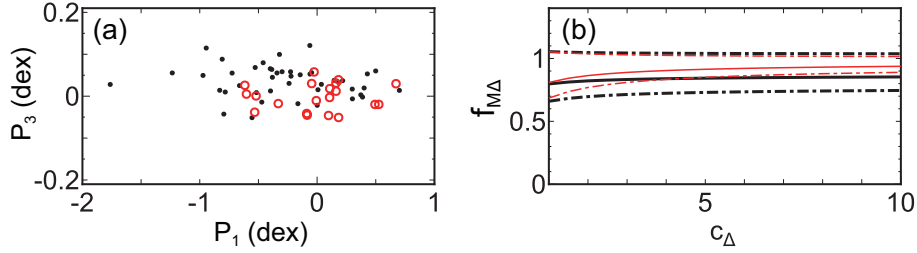
Figure 8. (a) Cross sections of the fundamental plane. Red open circles are the CLASH clusters (CFP) and black dots are the X-ray clusters (XFP). (b) Relation between f_{M\Delta} and concentration parameter c_\Delta . Solid lines are the fiducial relations and the dash-dotted lines show uncertainties. The difference of black and red lines come from the different assumptions of the plane shift (see [47]) (Figures are reconstructed from Figures 5 and 6 of [47]).
