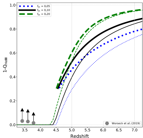
Figure 4. Redshift evolution of the double ionized helium fraction ( Q_{HeIII} ). Different line-types and colours refer to the predictions of our empirical modelling for different values of the f_{dc} parameter (as indicated in the legend). Thin lines refer to a model assuming homogeneous helium reionization, while thick lines show the predictions for the bubble model for the evolution of the ionization front of each luminous AGN/QSO (see text for more details). Grey symbols mark the observational determinations by Worseck et al. (2019).
