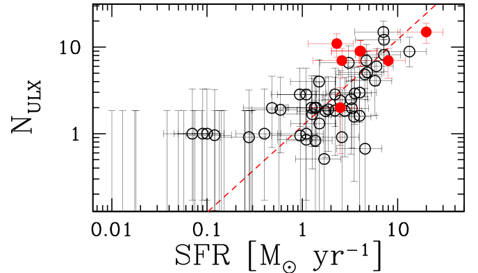
Figure 6. Number of ULXs per galaxy as a function of the host's SFR. Filled red circles are galaxies from this paper, while open black circles are from Mapelli et al. (2011). Error bars on the SFR are derived assuming a 50% uncertainty for all measures as in the previous papers. The red dashed line is the power-law fit obtained assuming that the index of the power law is equal to 1.
