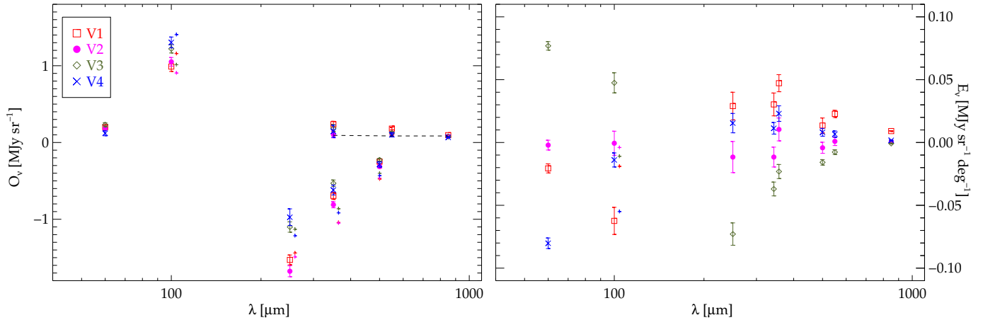
Fig. A.1. Left panel: offsets O_v . We also indicate with crosses estimates at 100 \mu\text{m} obtained summing the offset with LAB data and the residual zodiacal light contamination in IRIS maps as derived by Planck Collaboration XI (2014); estimates for SPIRE data using the SPIRE/HFI offsets from the zeroPointCorrection procedure in HIPE. The dashed line shows the offset derived by the Planck team on zodi-corrected maps (Planck Collaboration VIII 2014). Right panel: fitted gradient in ecliptic latitude E_v . Crosses show the gradient as derived from the correction described in Planck Collaboration XI (2014). To avoid cluttering, we have slightly displaced some symbols from their exact wavelength.
