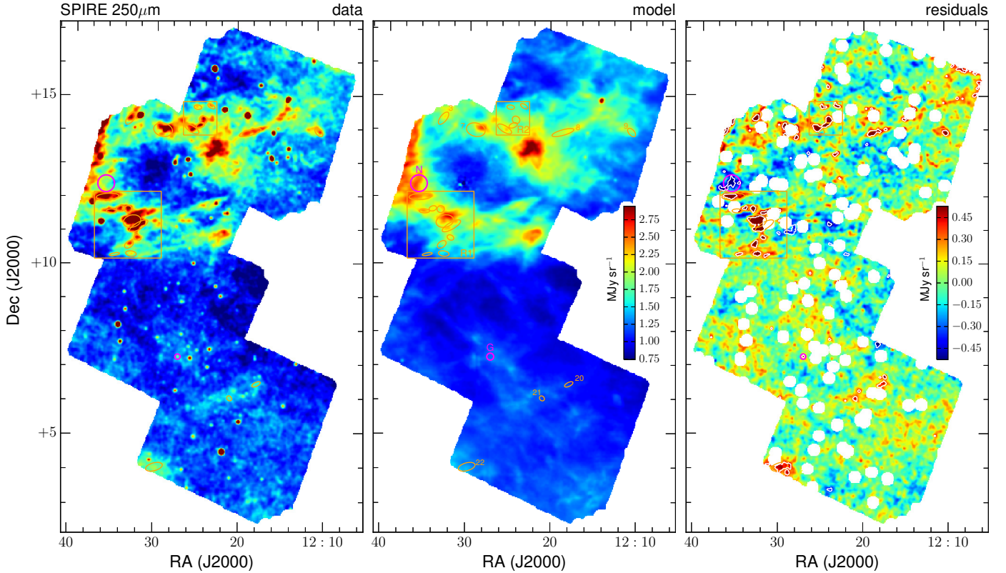
Fig. 8. Observations (left column), models (middle column), and residuals (right column) of the HeViCS field in the SPIRE 250 \mu\text{m} band. Observations and models were subtracted by the large-scale terms O_v + E_v \times (b - b_0) and are shown on the same color scale. The color scale of the residuals goes from -4 to 4\sigma_R (Table 1); round white areas show the object mask applied before the fitting, while white contours encircle the regions where residuals are larger than 3\sigma_R (excluded during the fitting). The orange numbered ellipses and square regions refer to the high positive residual regions listed in Table 3 and shown in Fig. 9. The magenta circle labeled “N” highlights a region with high negative residuals; the magenta circle labeled “G” is centered on an unmasked Virgo cluster galaxy.
