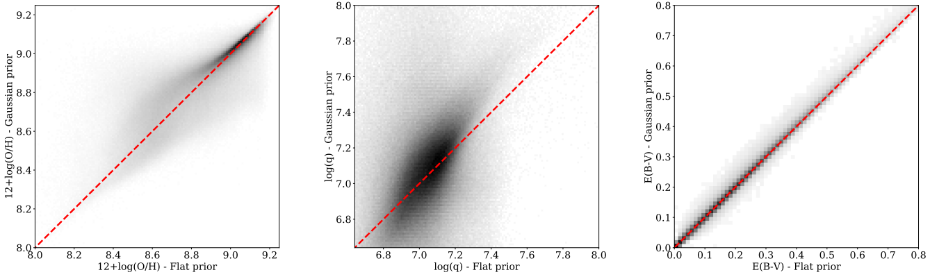
Fig. 7. Comparison between the results obtained with IZI with a flat (x-axis) and a Gaussian (y-axis) prior on the ionisation parameter, for metallicity, ionisation parameter, and gas extinction, respectively. The red dashed line represents the one-to-one relation.
