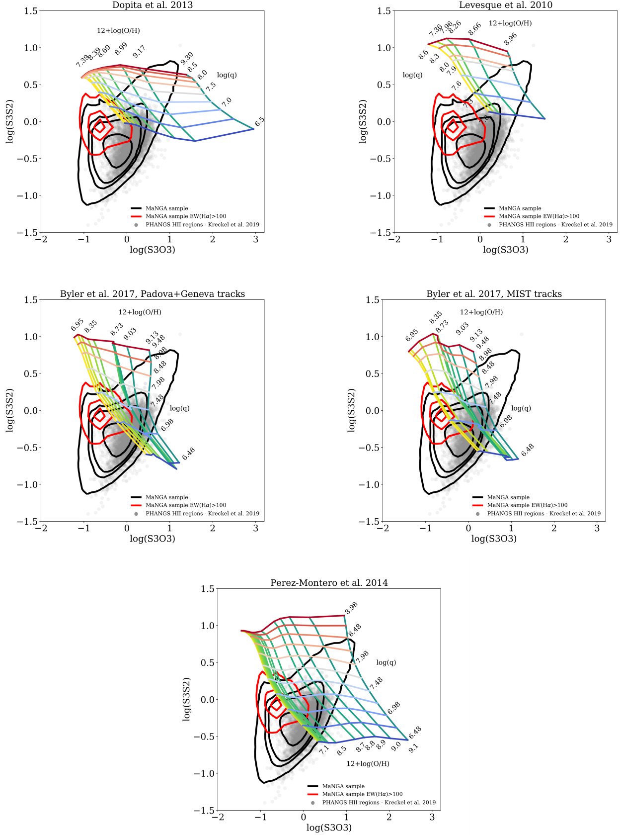
Fig. 3. [S\text{ III}]/[O\text{ III}] vs. [S\text{ III}]/[S\text{ II}] diagnostic diagrams introduced by Stasińska (2006) showing the density contours for all the star-forming spaxels of our sample (in black), with superimposed Dopita et al. (2013), Levesque et al. (2010), Byler et al. (2017) pdva+geneva, Byler et al. (2017) MIST, and Pérez-Montero (2014) models, respectively. Metallicity increases horizontally from yellow to green, while ionisation parameter increases vertically [redder means higher \log(q) and bluer lower \log(q) ]. The red contours correspond to the brightest MaNGA star-forming regions [EW(H\alpha) > 100] , while the grey dots are the H II regions analysed by Kreckel et al. (2019) with the PHANGS survey. Current photoionisation models fail to reproduce the observed [S\text{ III}] lines.
