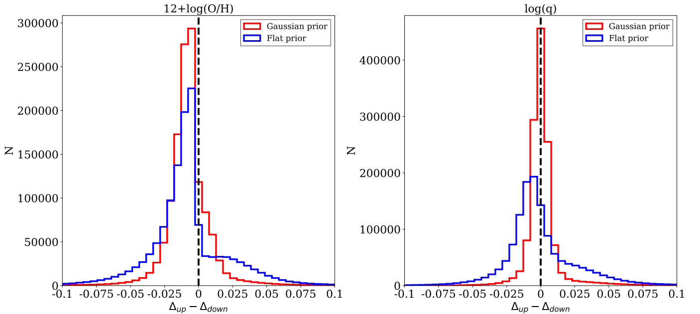
Fig. 8. Distribution of the difference between \Delta_{\text{up}} = 84\text{th} - 50\text{th} and \Delta_{\text{down}} = 50\text{th} - 16\text{th} for the metallicity (left panel) and ionisation parameter (right panel), in the case with a flat (in blue) and a Gaussian (in red) prior on the ionisation parameter, respectively, for all the spaxels of all the galaxies.
