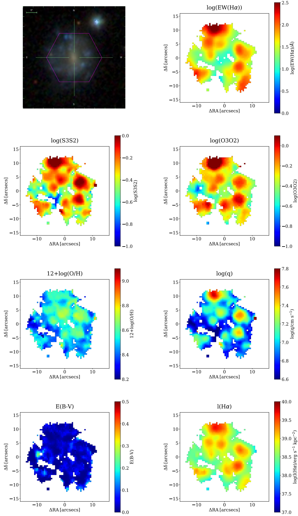
Fig. 10. Maps for the galaxy 8147–9102, with a stellar mass of \log(M_*/M_\odot) = 9.10 . The g-r-i image composite from SDSS with the MaNGA hexagonal FoV overlaid, equivalent width of \text{H}\alpha , S3S2, O3O2, IZI metallicity 12 + \log(\text{O}/\text{H}) , IZI ionisation parameter \log(q) , IZI gas extinction E(B-V) and \text{H}\alpha luminosity per spaxel L(\text{H}\alpha) maps are reported, respectively. East is to the left.
