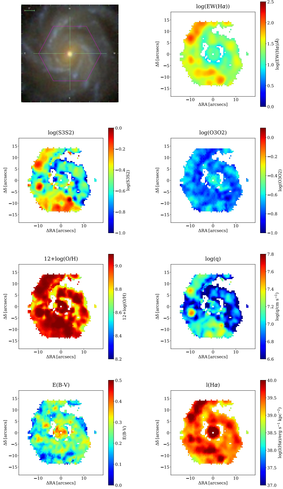
Fig. 11. Same as Fig. 10 but for the galaxy 9041-12701, with a stellar mass of \log(M_{\star}/M_{\odot}) = 10.93 .
