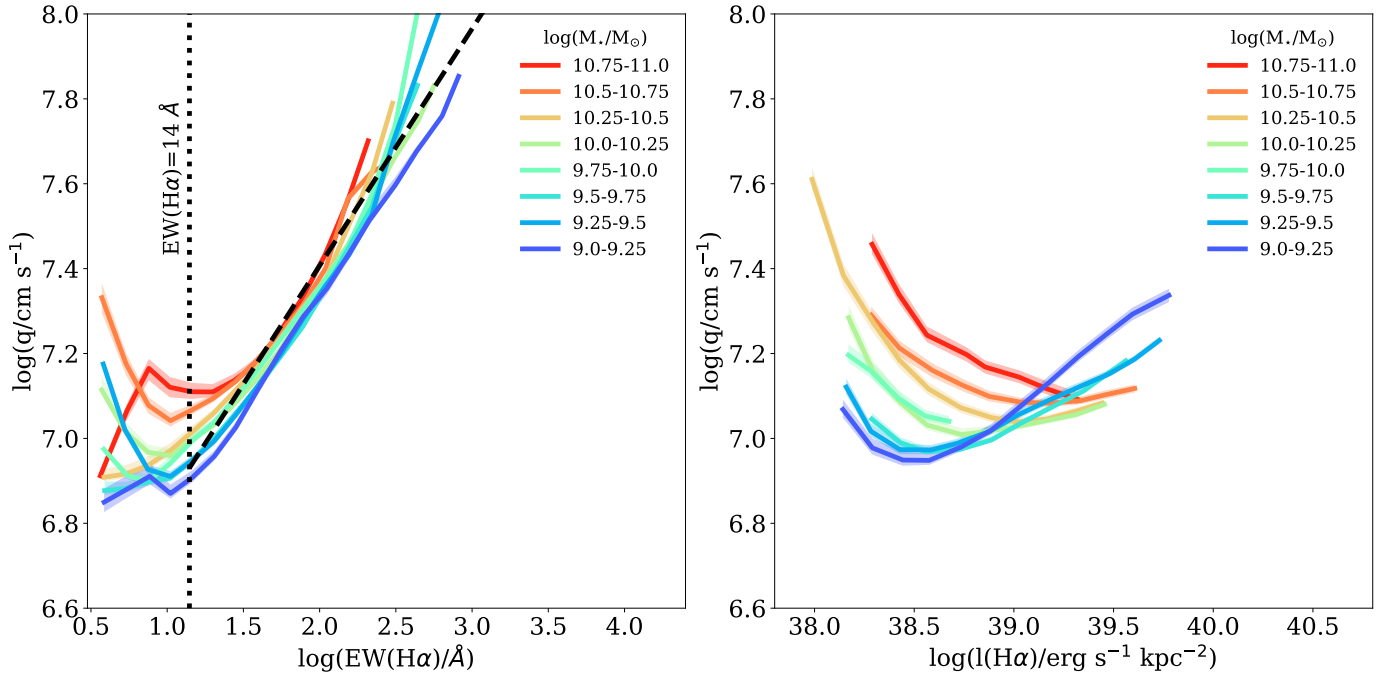
Fig. 14. Left: ionisation parameter \log(q) as a function of \text{H}\alpha equivalent width [\text{EW}(\text{H}\alpha)/\text{\AA}] dividing all the spaxels used in this work into bins of 0.15 dex and then separating the galaxies into bins of \log(M_*/M_\odot) . A nearly universal power-law relation is evident between the two quantities for \text{EW}(\text{H}\alpha) > 14 \text{\AA} (labelled with a dotted vertical line). Right: same as the left panel but for \text{H}\alpha luminosity per spaxel [l(\text{H}\alpha)/\text{erg s}^{-1}] . No universal relation is found in this case. The shaded regions represent the 16th and 84th percentiles of the distribution in each stellar mass bin taking into account the number of galaxies lying in the bin.
