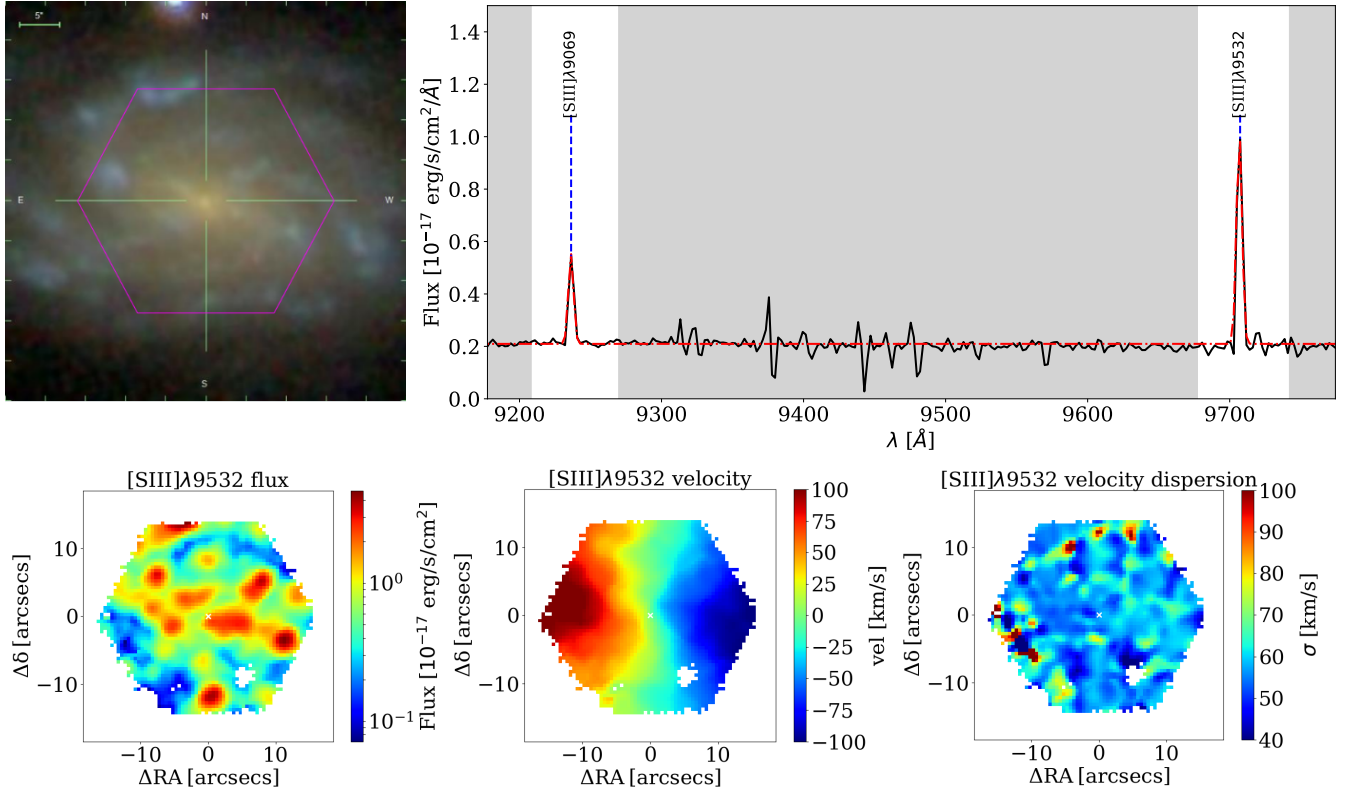
Fig. 1. Top left: g-r-i image composite from SDSS for MaNGA galaxy 8150–6103, with the MaNGA IFU hexagonal FoV overlaid. East is to the left. Top right: example of our fitting procedure for the [S III] lines for one representative spaxel in this example galaxy. The black solid line is the observed spectrum, while the dashed-dotted red line is the best fit. The regions in grey were masked before fitting. Bottom panels: [S III]λ9532 flux, velocity, and velocity dispersion maps of MaNGA galaxy 8150–6103.
