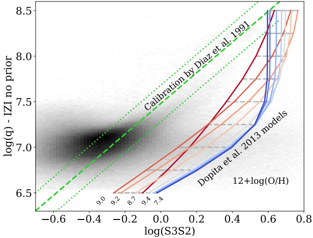
Fig. 6. Distribution of \log(q) as a function of \log(S3S2) inferred with IZI with a flat prior on the ionisation parameter, shown in shades of grey. The green dashed line shows the \log(q) values obtained with Eq. (2) (Diaz et al. 1991), while the green dotted lines represent the \pm 0.2 dex scatter around this relation. The models of D13 are shown in colour (red to blue, going from higher to lower metallicity).
