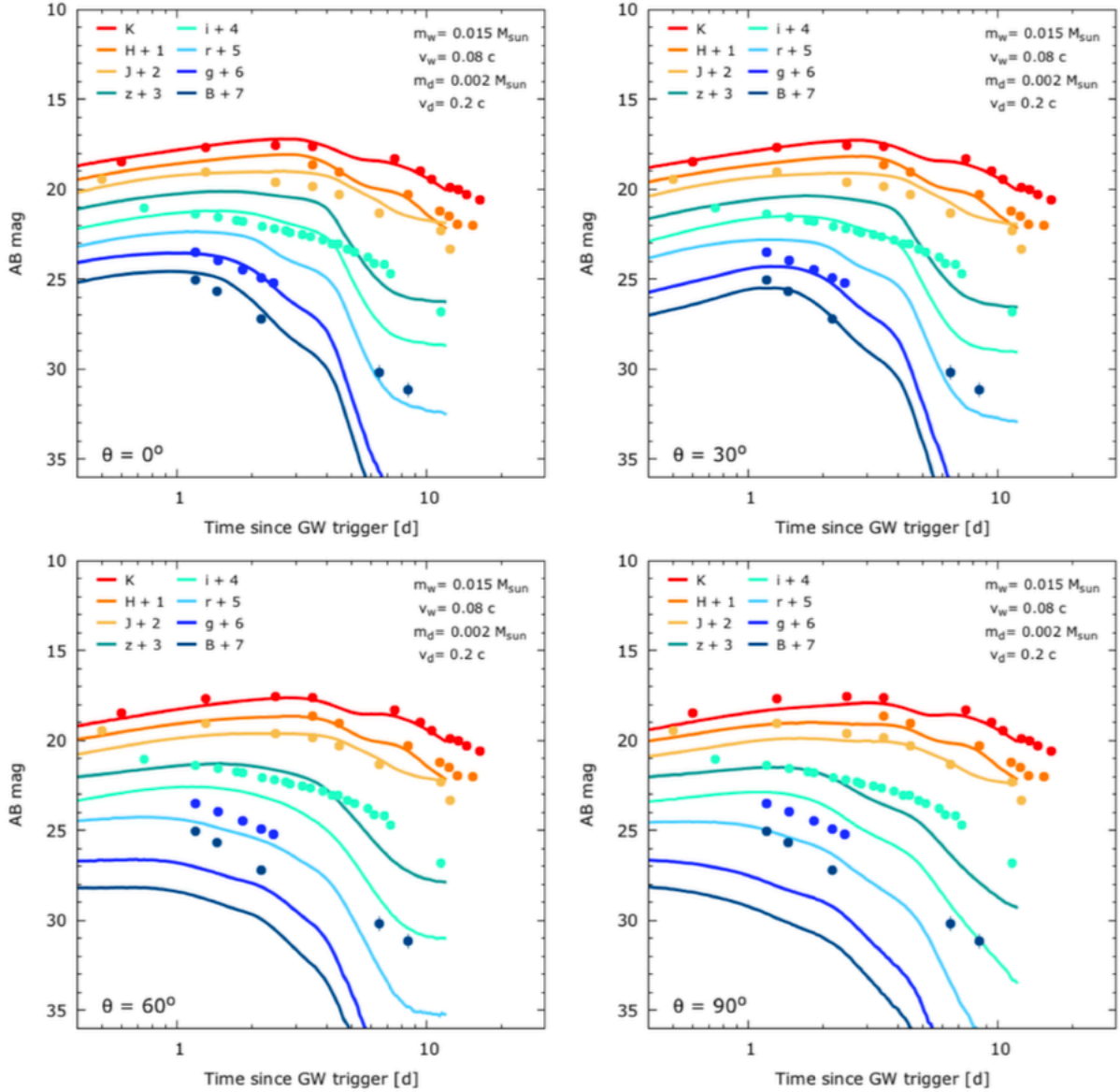
Extended Data Figure 4 - Kilonova light curves as a function of the viewing angle
