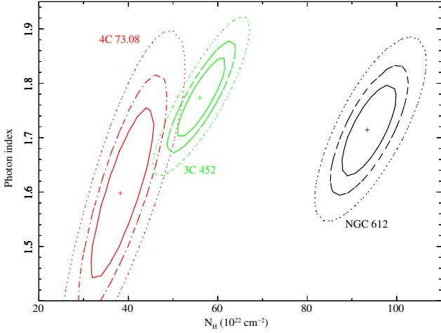
Figure 3. Contour plots of the column density N_H versus the photon index of the primary power law (MYTORUS model, see Table 3) for NGC 612 (black), 4C 73.08 (red) and 3C 452 (green). Solid, dashed and dotted lines correspond to 68 per cent, 90 per cent and 99 per cent confidence levels, respectively.
