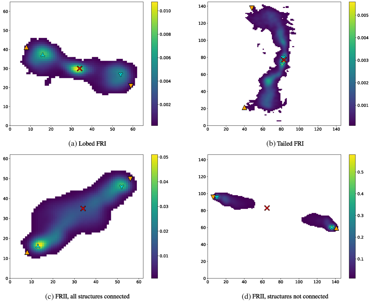
Figure 2. Examples of sources classified as FRI and FR II. The plots are produced as output by the classification code, and detail the pixel distances from the optical host (red X) to the first and second-brightest peak of emission excluding the core (d1 and d2 as per Fig. 1; inverted and non-inverted cyan Y, respectively), and the maximum extent of the source in both directions (D1 and D2 as per Fig. 1; up and down pointing orange triangles, respectively for the directions to the brightest and second-brightest peak). The scale is in pixel coordinates, with a scale of 1.5 arcsec per pixel. The colour bar represents flux units in \text{Jy beam}^{-1} .
