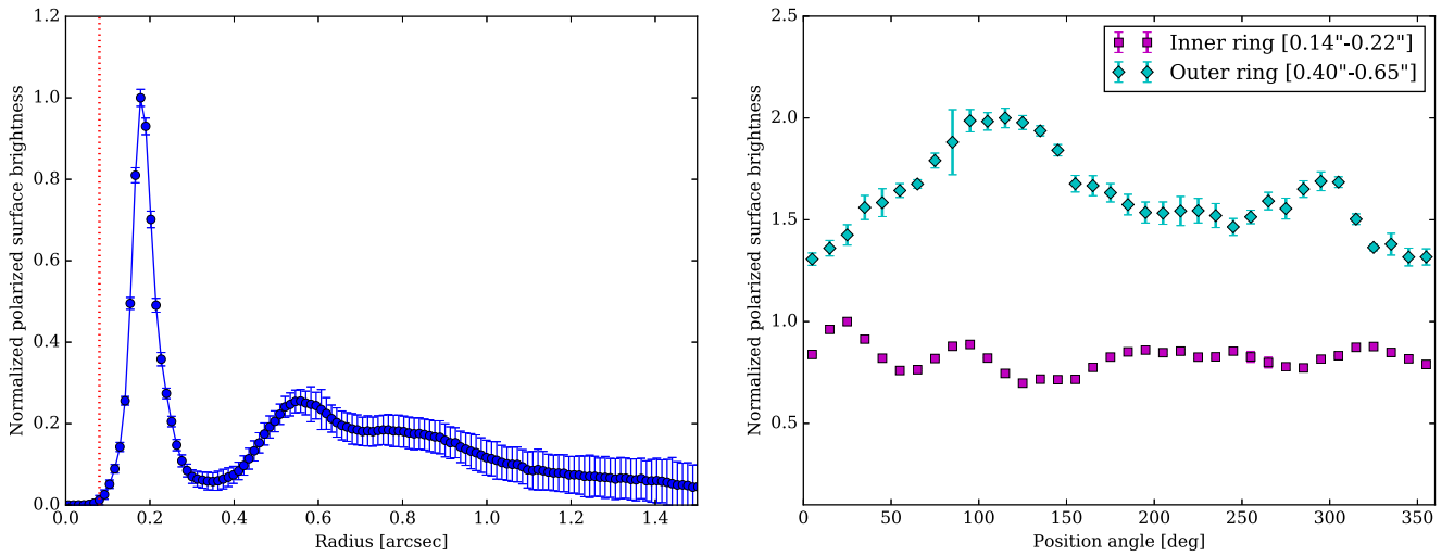
Figure 3. Normalized radial (left) and azimuthal intensity profiles (right) obtained after deprojection of the r^2 -scaled J -band Q_\phi image. The radial cut is obtained after azimuthally averaging and normalized to the maximum brightness of the inner ring. The red vertical dotted line is the limit of our IWA. The normalized azimuthal cuts are obtained after averaging radially between 0''.14 and 0''.22 (inner ring, purple squares) and between 0''.4 and 0''.65 (outer ring, green diamonds). The green curve is shifted vertically for clarity. The plotted error bars are the standard deviation in each bin in the U_\phi image on a pixel basis.
