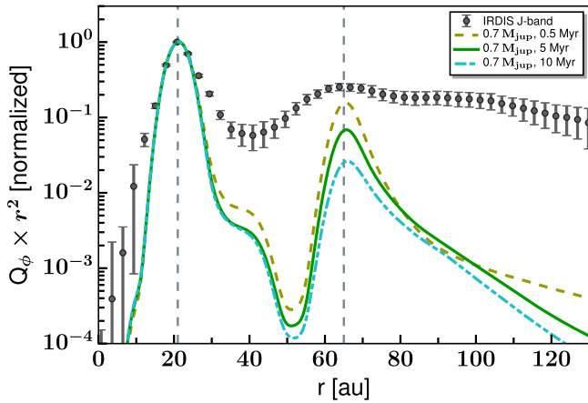
Figure 14. Comparison of surface brightness radial profiles of the Q_\phi \times r^2 model image at the J band for different dust evolution timescales. The values are scaled by the square of the distance from the central star in order to compensate for the falloff of the stellar irradiation. The vertical dashed lines mark the positions of the brightness peaks.
