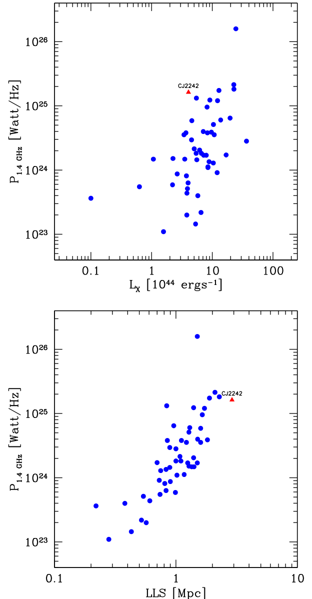
Figure 4. Radio halo power at 1.4 GHz versus the cluster X-ray luminosity in the 0.1–2.4 keV band (top) and versus the largest linear size of the radio halo measured at 1.4 GHz (bottom). Full dots are observed clusters taken from the literature. We added to the compilation by Feretti et al. (2012) new radio haloes in merging galaxy clusters revealed through pointed interferometric observations at \simeq 1.4 GHz (Govoni et al. 2012; van Weeren et al. 2012; Giovannini et al. 2013; Martinez Aviles et al. 2016; Shakouri, Johnston-Hollitt & Pratt 2016; Parekh et al. 2017). A red triangle marks the cluster CJ2242.
