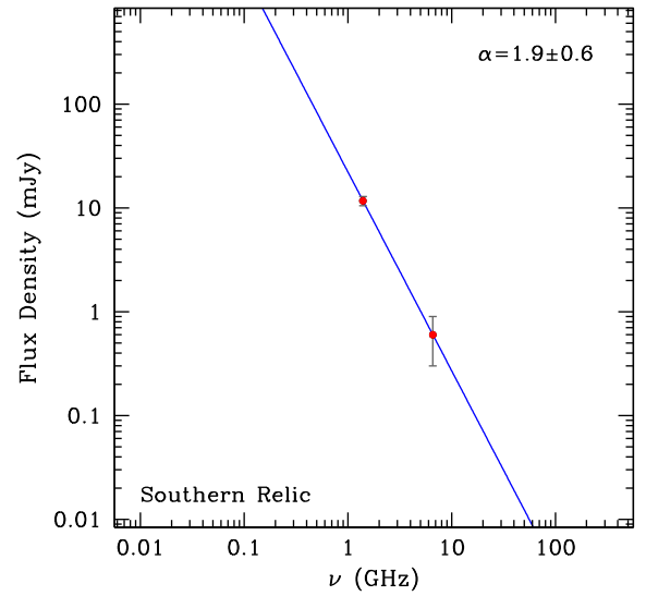
Figure 10. Total flux measurements of the southern relic obtained with the SRT observations.
