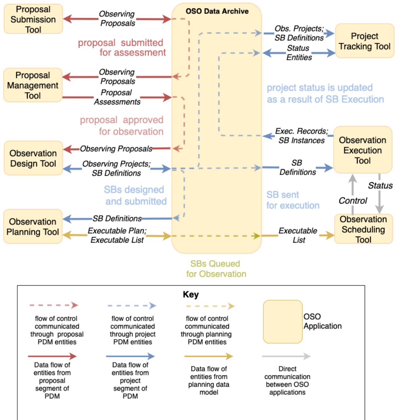
Figure 2. Overview of OSO tools and their relationship with the Data archive.
