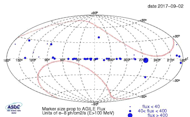
Fig. 4 The large AGILE-GRID FoV in spinning on a particular day. The sky regions not accessible for solar panel constraints are delimited in red, and indicate the mean daily sun and anti-sun positions
