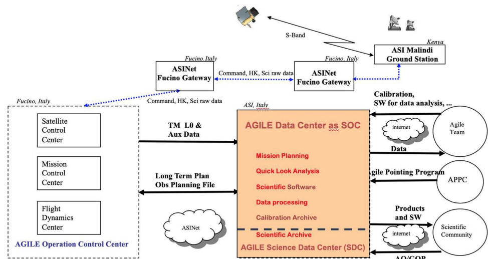
Fig. 2 Ground segment (GS) architecture of the AGILE space mission. The AGILE data center acts both as a science operation center (SOC) and as a science data center (SDC)
