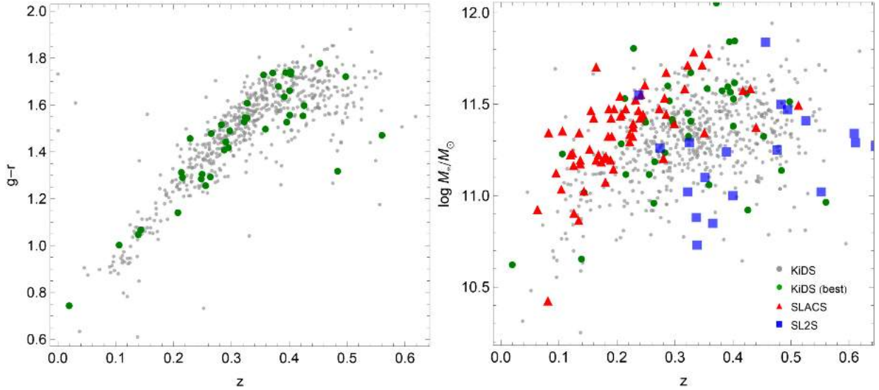
Figure 9. The g-r observer-frame colour, corrected for Galactic extinction (left-hand panel) and stellar mass (right-hand panel) versus redshift for a subsample of 659 ConvNet candidates with spectroscopic redshift available (grey dots). The subsample of best candidates with a visual score larger than 28 is shown as green points. Stellar masses (see Section 4.1) are compared with the SLACS sample from Auger et al. (2009, red triangles) and the SL2S sample from Sonnenfeld et al. (2013b, blue squares).
