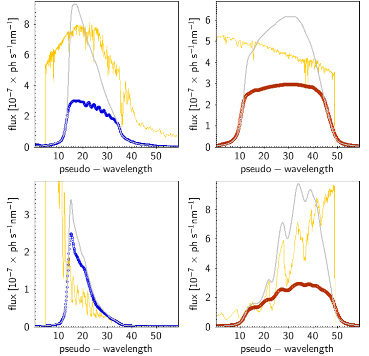
Fig. 45. Examples of heavily saturated spectra taken from the NGSL set: sources Gaia DR3 2067518817314952576 (top) with G = 2.11 and G_{BP}-G_{RP} = 0.99 and Gaia DR3 2106630885454013184 (bottom) with G = 2.36 and G_{BP}-G_{RP} = 2.42 . Colour coding and symbols are the same as in Fig. 21.
