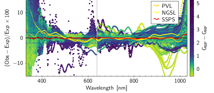
Fig. 23. Difference between observed and expected mean flux as a function of wavelength for BP and RP sampled mean spectra. A grey calibration has been applied to spectra. The three curves represent the smoothed medians for SPSS (red), PVL (orange), and NGSL (yellow). The colourmap encodes the G_{BP}-G_{RP} colour index.
