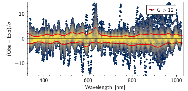
Fig. 37. Normalised residuals between ECS and reference fluxes for sources with G > 12 . The two red curves represent the P_{16} and P_{84} percentile distributions smoothed by a Gaussian with \sigma = 10 nm. The \pm 2 levels are also plotted as horizontal dashed black lines.
