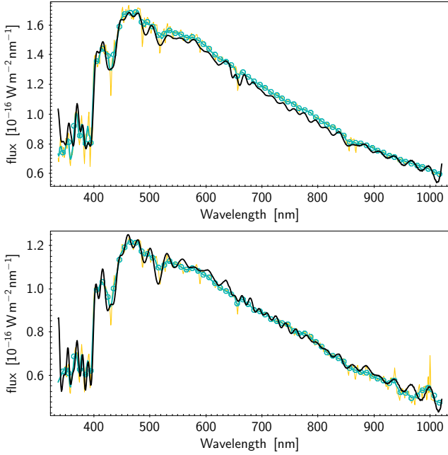
Fig. 34. Comparison between ECS and model SED for source GaiaDR3 1399559249961569792 ( top ) and source GaiaDR3 2323394345824851584 ( bottom ), two SPSSs of similar spectral type and magnitude. The colour coding and symbols are the same as in Fig. 32.
