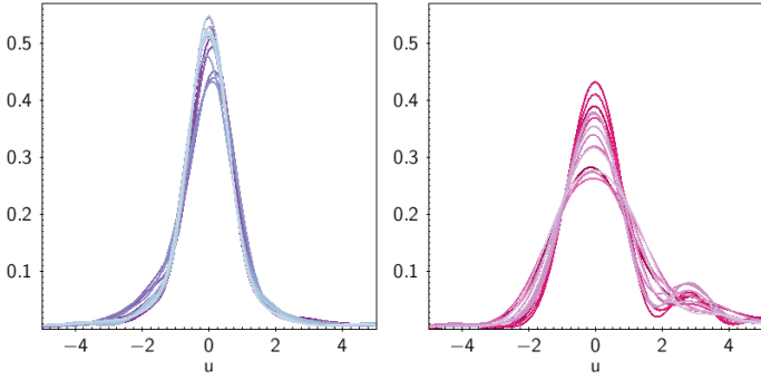
Fig. 3. Example of pre-launch nominal monochromatic LSF computed at wavelength \lambda = 440 nm (left) and \lambda = 800 nm (right). Different curves represent the LSF for each FoV/CCD row combination.
