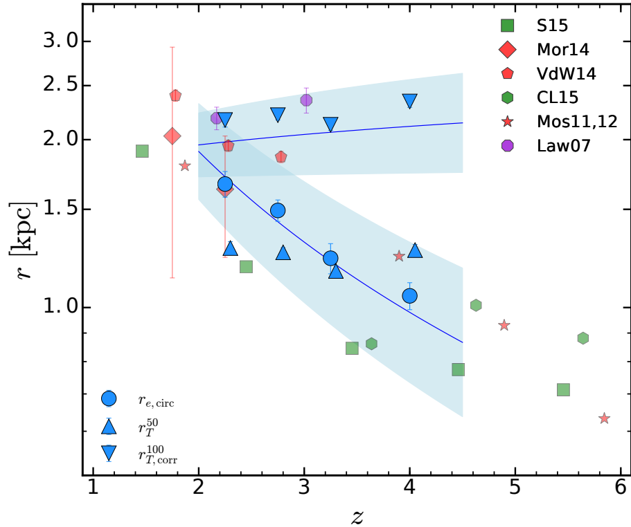
Fig. 22. Compilation of size measurements at different redshifts for a number of different studies. First, in blue we show the measurements of this paper. Circles are taken from the GALFIT effective radius, and the triangles and inverted triangles are from r_T^{50} and r_T^{100} respectively. The blue solid lines and respective shaded regions show the derived evolution for r_{e,circ} and r_T^{100} . Each other color represents a different sample selection (green for luminosity-selected samples, red for stellar-mass-selected samples, and purple for a different selection) and each symbol represents a different study. They are squares (Shibuya et al. 2015), 0.3L_* < L < 1L_* ; diamonds (Morishita et al. 2014), 10.0 < \log_{10}(M_*/M_\odot) < 10.5 ; pentagons (van der Wel et al. 2014), 10.0 < \log_{10}(M_*/M_\odot) < 10.5 ; hexagons (Curtis-Lake et al. 2016), 0.3L_* < L < 1L_* ; stars (Mosleh et al. 2011, 2012), 9.5 < \log_{10}(M_*/M_\odot) < 10.4 ; octagons (Law et al. 2007), spectroscopic sample, no mass or luminosity selection.
