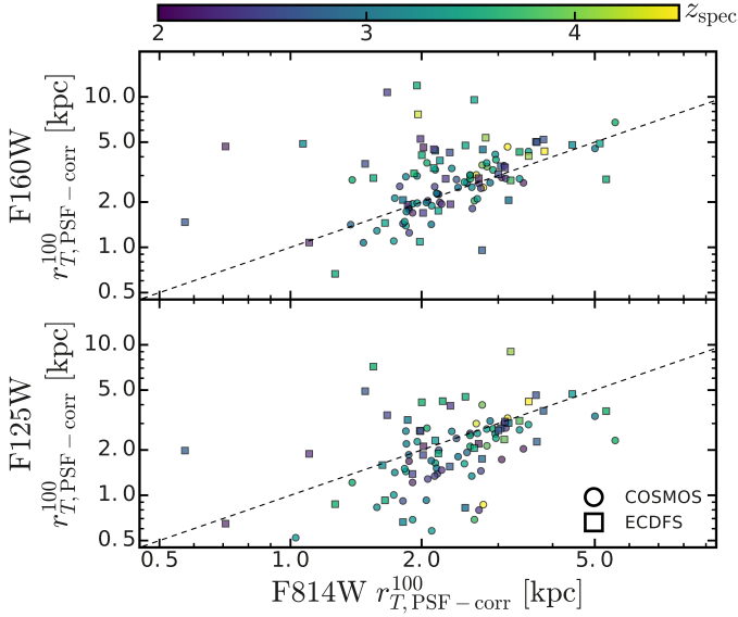
Fig. 11. Comparison of r_{T,\text{PSF-corr}}^{100} size measurements for a subset of VUDS galaxies at 2 < z < 4.5 with available F814W and F160W/F125W images from CANDELS. Results are split into two bands: F160W in the top panel and F125W in the bottom panel. Circles and squares refer to COSMOS and ECDFS respectively. The dashed black line shows where the two radii are equal. The symbols are color coded according to their spectroscopic redshift, and the mapping is shown in the colorbar at the top of the plots.
