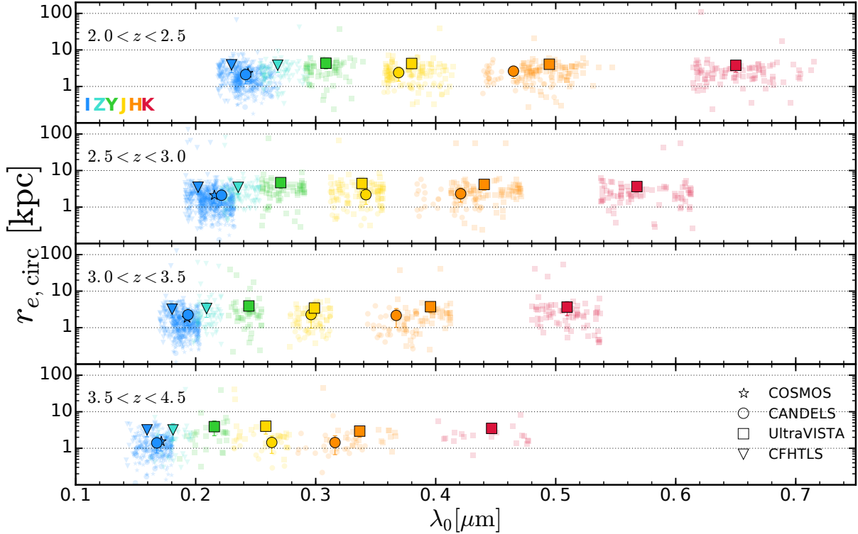
Fig. 5. Measured sizes as a function of wavelength for galaxies with \log_{10}(M_{\star}) > 9.5 at 2 < z < 4.5 in the COSMOS field. Different symbols correspond to different surveys (symbol coding in the bottom panel ) and different colors to different observed bands (color coding in the top panel ). Each point represents the size of a given galaxy at the rest-frame wavelength of the pivot of the filter.
