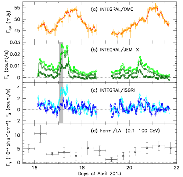
Figure 14: Light curve of MKN 421 in April 2013, see Pian et al. (2014)
