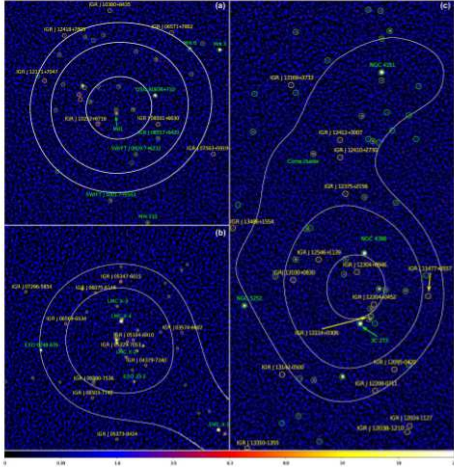
Figure 2: Hard X-ray maps of the M81, LMC and 3C 273/Coma fields as in Mereminskiy et al. (2016)
