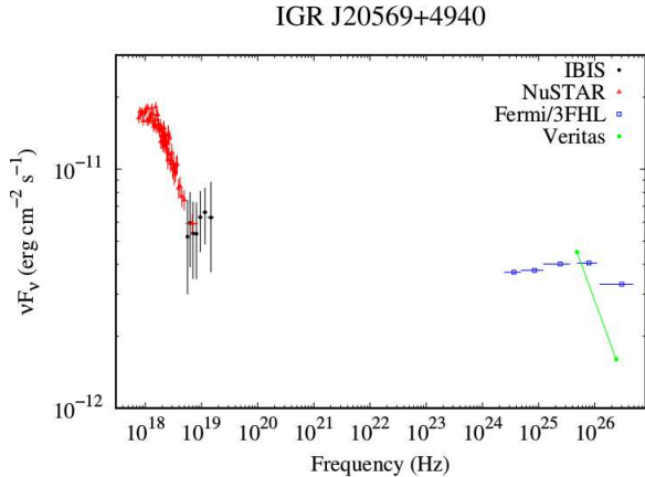
Figure 16: Spectral Energy Distribution of IGR J20569+4940 obtained assembling unpublished NuSTAR observation performed in November 2015 with the average INTEGRAL and Fermi /LAT spectra with the addition of the reported TeV data (courtesy of F. Ursini).
