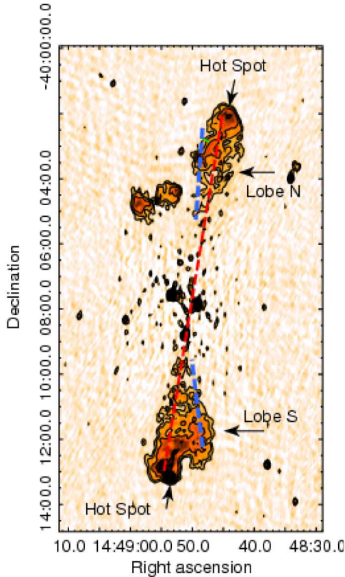
Figure 13: Radio 610MHz GMRT full resolution image of IGR J14488-4008 as in Molina et al. (2015)
