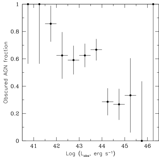
Figure 8: Observed fraction of absorbed AGN as a function of observed hard X-ray luminosity. From (Sazonov et al., 2015).
