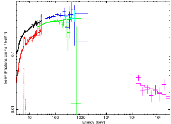
Figure 5: Combined INTEGRAL and (non-simultaneous) Fermi /LAT unfolded spectrum of Cen A as in Beckmann et al. (2011). The data are modelled by a double broken power-law with individual normalisation for the data of different epochs. The highest energy bins for IBIS/ISGRI and SPI are only upper limits.
