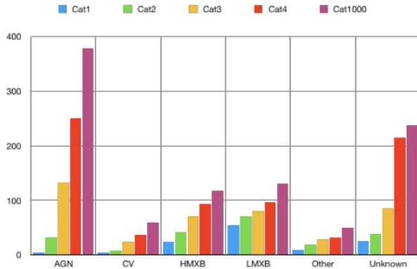
Figure 1: Evolution of source type and number through the five INTEGRAL IBIS/ISGRI catalogs produced to date (courtesy of A. J. Bird)
