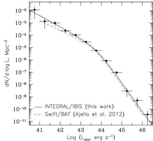
Figure 9: Observed hard X-ray luminosity function of local AGN (circles) fitted by a broken power law (solid line). For comparison, the luminosity function based on the Swift /BAT survey (Ajello et al., 2012) is shown by the dashed line. From (Sazonov et al., 2015).
