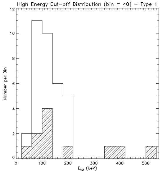
Figure 6: High-energy cut-off distribution of the entire sample from Malizia et al. (2009). The diagonally hatched histogram represents sources for which only lower limits of E_{\text{c}} are available.
