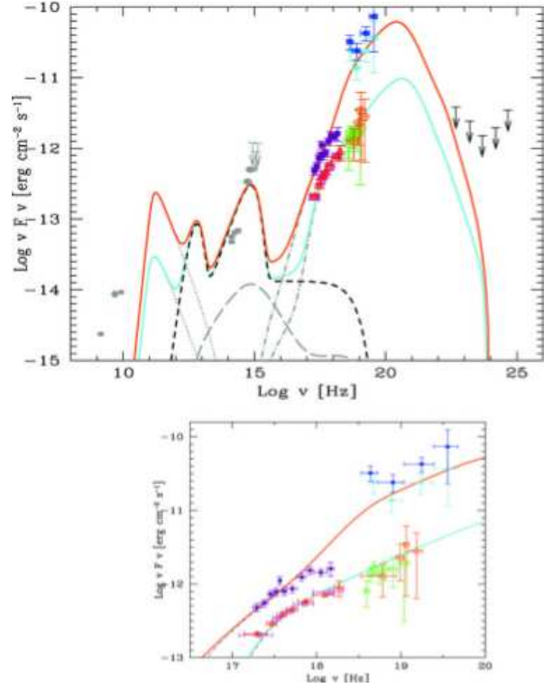
Figure 15: Top: spectral energy distribution of IGR J22517+2217. Grey circles and arrows represent archival radio/optical/UV data from NED. Red triangles and magenta squares represent XIS 0 and XIS 3 data, green circles and orange pentagons represent PIN and BAT quiescent data respectively, while black arrows are Fermi upper limits in five bands. Filled violet squares represent XRT data, filled cyan diamonds and blue pentagons represent IBIS and BAT flare data respectively. The solid cyan and orange curves are the results of modelling of the quiescent and flaring states, respectively. With grey lines we show the different components of non-thermal emission: synchrotron (dotted), synchrotron self-Compton (long-dashed) and external Compton (dotdashed). The black dashed line corresponds to the thermal emission of the disc, the IR torus and the X-ray disc corona. The model does not account for radio emission, produced from much larger regions of the jet. Bottom: enlargement in the X-ray energy range for the two SEDs. Symbols as in the top panel. Figure from Lanzuisi et al. (2012)
