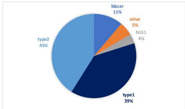
Figure 4: Pie chart of the main classes of AGN in the INTEGRAL sample.
