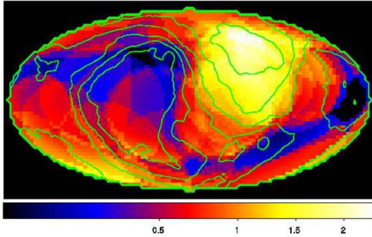
Figure 12: 2D-map (in Galactic coordinates) of the AGN number density in the local Universe compared to that of normal galaxies. See (Krivonos et al., 2007) for details.
