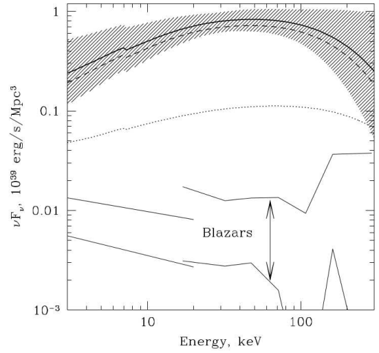
Figure 11: Cumulative spectrum of the local Seyfert galaxies, based on INTEGRAL and RXTE data (solid line with the corresponding hatched uncertainty region). The dashed and dotted lines show the contributions of low- ( < 10^{43.5} erg s ^{-1} ) and high- ( > 10^{43.5} erg s ^{-1} ) luminosity AGN, respectively. The estimated contribution of blazars is also shown. From (Sazonov et al., 2008a).
