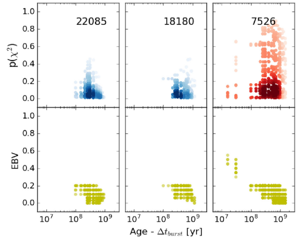
Figure 2. Probability ( p(\chi^2) , upper panels) and E(B - V) (lower panels) as a function of [\text{age} - \Delta t_{\text{burst}}] of all the possible solutions in the SED-fitting process, for three red and dead candidates in the reference sample (IDs 22085, 18180 and 7526, chosen as examples of three levels of robustness in the selection; see also Fig. 4; and the plot for the full TH sample is in Appendix D). The colours of the dots in the probability panels refer to the belonging of the source to the selection with (blue) or without (red) the inclusion of nebular lines. The dots (i.e. the models) are shaded as a function of their density. All the solutions have age > \Delta t_{\text{burst}} , as required to be classified as passive in this approach. Galaxies excluded from the selection, on the other hand, have been fitted by at least one model with age \leq \Delta t_{\text{burst}} , i.e. still star-forming, with a probability p > 5 per cent (not shown). [A colour version of this figure is available in the online version.]
