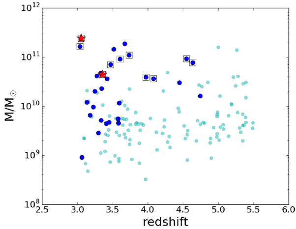
Figure 3. Redshift versus mass distribution of the red and dead selections. Cyan points refer to objects having z < 5.5 and a passive best-fitting solution (both in the fit including emission lines and in the one without them), but excluded from the reference sample because of the existence of different, non-passive solutions with probability larger than 5 per cent; blue dots: reference sample (30 candidates surviving the probabilistic selection; the void squares mark the 10 sources selected also using the library including nebular lines emission); red stars: the two candidates surviving the free- z fitting. See the text for more details. [A colour version of this figure is available in the online version.]
