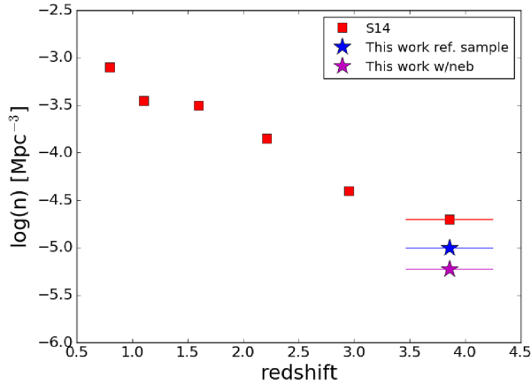
Figure 5. Number density of red and dead candidates with \log[M/M_{\odot}] > 10.6 in the redshift bin 0.65 < \log(1+z) < 0.72 , from this work (blue star: reference sample; magenta star: ‘emission lines’ selection), compared to the results by S14 (red squares). Our mass estimates are corrected to match the analysis by S14, who assumed a Chabrier IMF rather than a Salpeter IMF. See the text for more details. [A colour version of this figure is available in the online version.]
