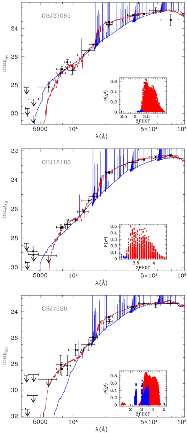
Figure 4. Fitted SEDs of the three candidates reported in Fig. 2 in the reference sample, in the free- z fit. In each panel, the red line is the best passive solution at the CANDELS photometric redshift, and the blue line is the best star-forming solution (at a different redshift); the dots in the inner panel refer to the corresponding probabilities. Top: ID22085, a strong candidate surpassing all the selection criteria: the best star-forming solution (obtained at z \simeq 3.4 ) has probability p < 5 per cent, so this object can safely be considered passive even letting its redshift freely vary in the fit. Middle: ID18180, despite having mostly passive solutions with very high probabilities, it also has a few star-forming solutions with p > 5 per cent (at z \simeq 3.1 ), so it is formally excluded from the most stringent selection. Bottom: ID7526 (which is part of the reference sample, but fails the emission line fit selection) has many high-probability star-forming solutions at various redshifts. [A colour version of this figure is available in the online version.]
