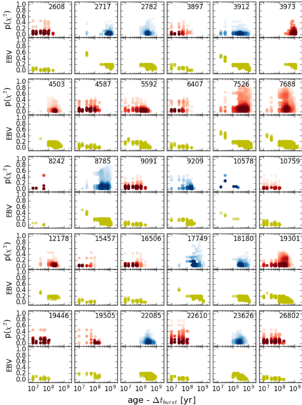
Figure D1. Probability and dust extinction as a function of [\text{age} - \Delta t_{\text{burst}}] for all the possible solutions in the SED-fitting process, for all the candidates in the TH selection. For each candidate, indicated by its ID, two panels are shown. In the upper one, dots represent the probability p(\chi^2) of each model solution; the colours of the dots refer to the belonging of the source to the selection with (blue) or without (red) the inclusion of nebular lines; the dots (i.e. the models) are shaded as a function of their density. The lower one shows the corresponding values of the E(B - V) . All the solutions have \text{age} > \Delta t_{\text{burst}} , as required to be classified as passive in this approach. Galaxies excluded from the selection, on the other hand, have been fitted by at least one model with \text{age} \leq \Delta t_{\text{burst}} , i.e. still star-forming, with a probability p > 5 per cent (not shown). [A colour version of this figure is available in the online version.]
