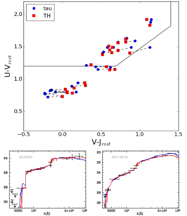
Figure 7. In the top panel we show the shifts on the UVJ diagram of the objects in the reference sample, when fitted with different libraries of models. Blue dots: exponentially declining ( \tau ) library; red squares: TH library. The shifts are small ( \sim 0.3 \Delta\text{mag} ) and typically more pronounced in the V - J colour. The bottom panels show two examples explaining the described trend: the fitted SEDs substantially coincide in the optical – NIR, but differ in the IRAC region. See the text for more details. [A colour version of this figure is available in the online version.]
