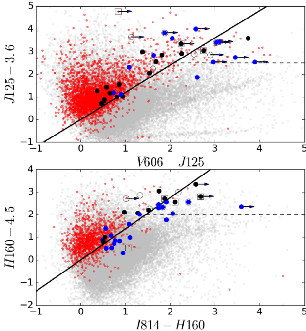
Figure 8. Diagnostic colour-colour diagrams. In both panels, grey dots are the whole G13 catalogue, and red dots are the sources having z_{\text{CANDELS}} in the interval of interest for the corresponding diagnostic diagram: 2.5 < z < 3.5 for the VJ plot (top panel), 3.5 < z < 4.5 for the iH plot (bottom panel). Black and blue dots are the reference sample red and dead candidates, respectively, having redshift within the interval of interest and outside it (arrows are upper limits). Empty squares and circles refer to the \tau selection (Section 5), again, respectively, having redshift within the interval of interest and outside it. [A colour version of this figure is available in the online version.]
