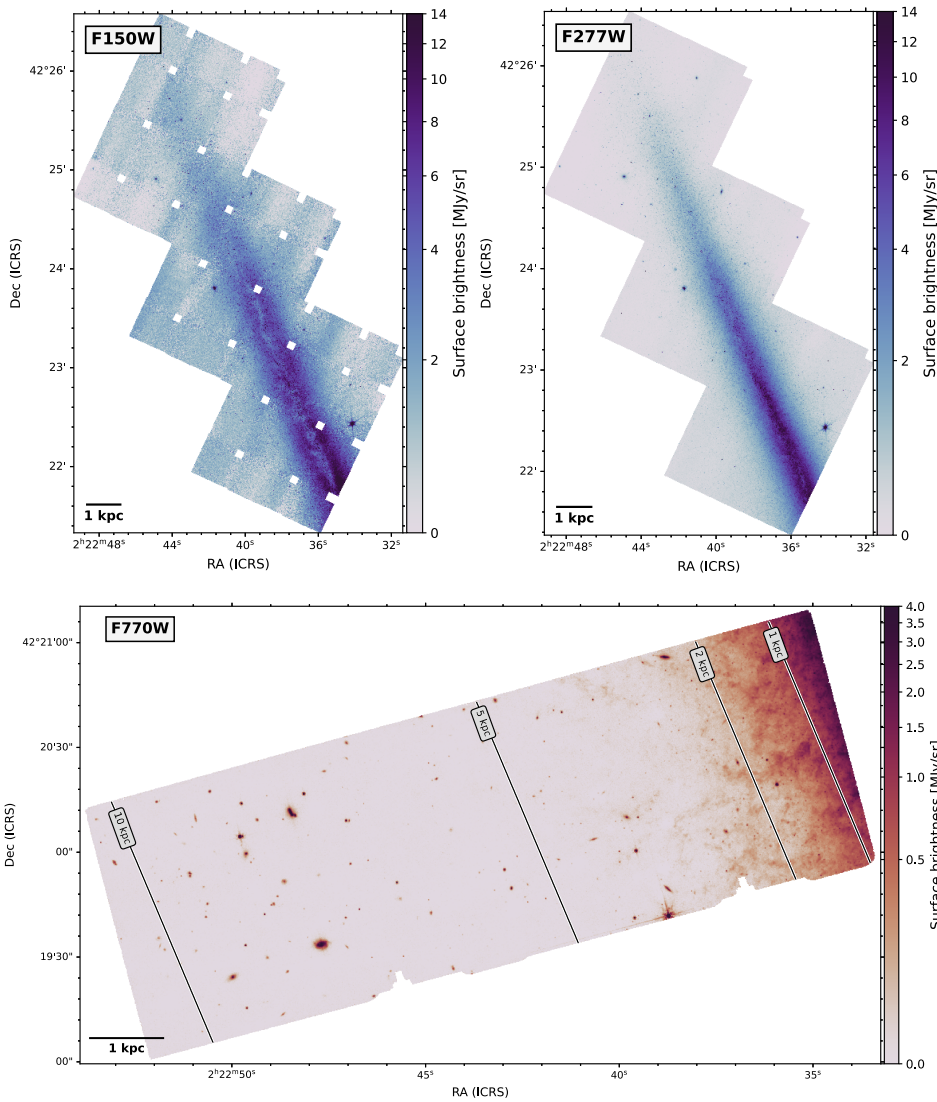
Fig. 2. Final JWST NIRCам and MIRI images. Top left: NIRCам F150W data, at native \sim 0.05'' resolution. The mid-plane shows conspicuous absorption. The background in that band shows large discrepancies, due to the difficulty to correct for both large structure stripes and offsets between the individual dithers. The small squares are gaps in the dither-pattern coverage. Top right: NIRCам F277W data, at native \sim 0.092'' resolution. Some absorption is visible in the mid-plane, and the image shows a much smoother background than for the F150W mosaic. Bottom: MIRI F770W data, at native \sim 0.25'' resolution, with radial distance indicators at 1, 2, 5, and 10 kpc from the mid-plane. The mid-IR image shows many filamentary structures as far out as \sim 4 kpc.
