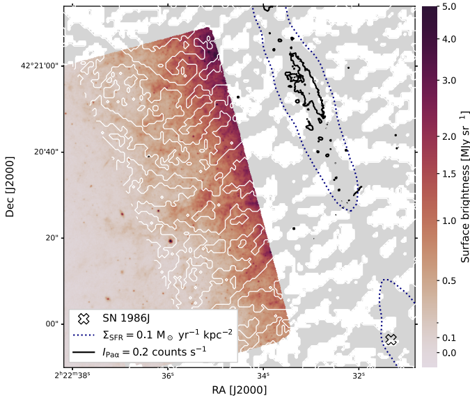
Fig. 8. IRAC 8 \mu m unsharp-mask, shown in grey, with the MIRI image overlaid. The white contours show the continuation of the structures in the IRAC unsharp-mask, nicely following some of the structure visible in high-resolution in the MIRI map. We show contours of star formation rate surface density of 0.1 \text{ M}_{\odot} \text{ yr}^{-1} \text{ kpc}^{-2} derived from the MIPS-24 \mu m image, and intensity of Pa- \alpha , another tracer of recent star formation. The cross at the bottom-right shows the location of SN1986J.
