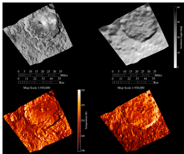
Fig. 2. Equirectangular projection of a portion of Occator crater, observed by VIR during the HAMO phase (0.38 km/px) in the local morning (9.5 h LST), using the same four-panels scheme adopted in Fig. 1. A horizontal scale bar accounts for the size of the features observed in the scene. Near the center of the crater, some structures are revealed with thermal contrast not due to the local topography, which correspond to the area of the central (main) bright spot. In contrast, the secondary (smaller) bright spots located in the eastern side of the floor do not show any substantial thermal contrast. The thermal behavior of the bright spots in Occator can be attributed both to their albedo and the compactness of the material they are made of. Daytime surface temperatures in the bright spots are overall incompatible with stable exposure of water ice.
