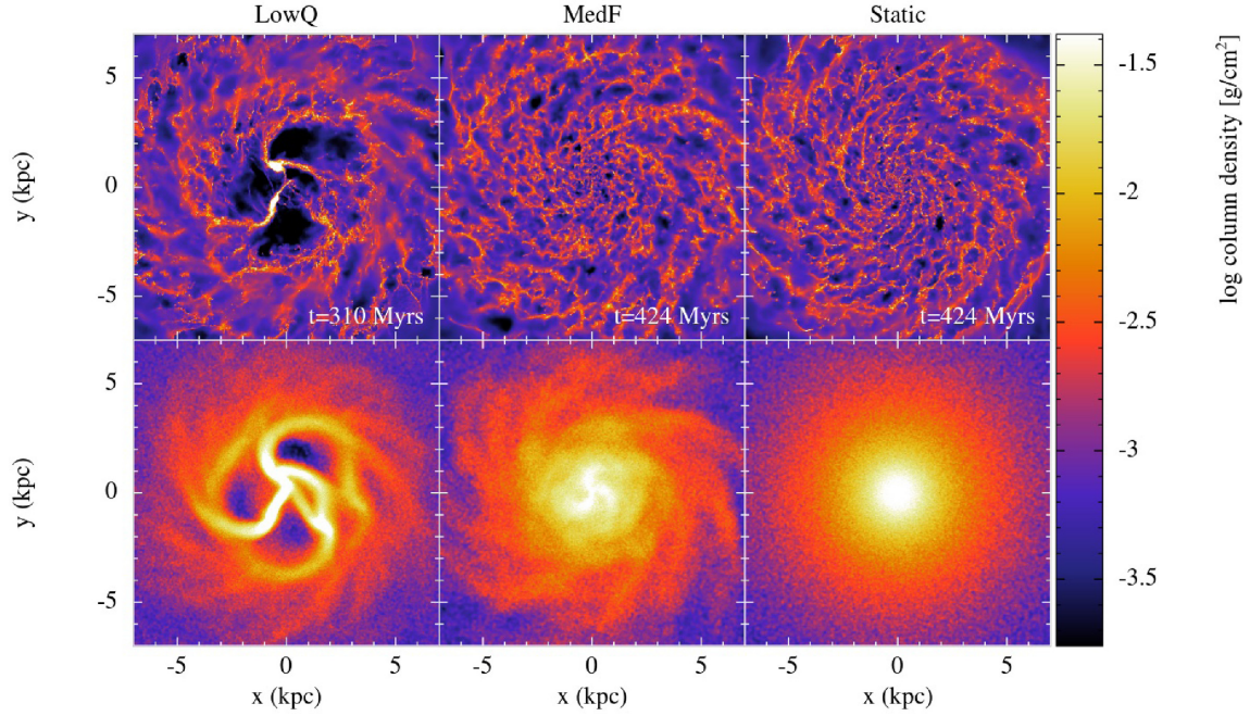
Figure 4. The gas (top) and stellar (lower) distributions are shown for models with different Q : LowQ (left), MedF (centre), and Static (right) with Q \sim 0.5 , 1, and \infty , respectively. For Q \sim 0.5 , there are very strong arms in both the gas and stars. For the static stellar disc, there are many arms in the gas, and no clear spiral structure, as would be expected from gravitational instabilities only in the gas. For Q \sim 1 , there is slightly clearer large-scale structure in the gas (this is more true for other star formation efficiencies, as we show in Fig. 5). The LowQ model is shown at an earlier time, as this model was so unstable it was difficult to run for long.
