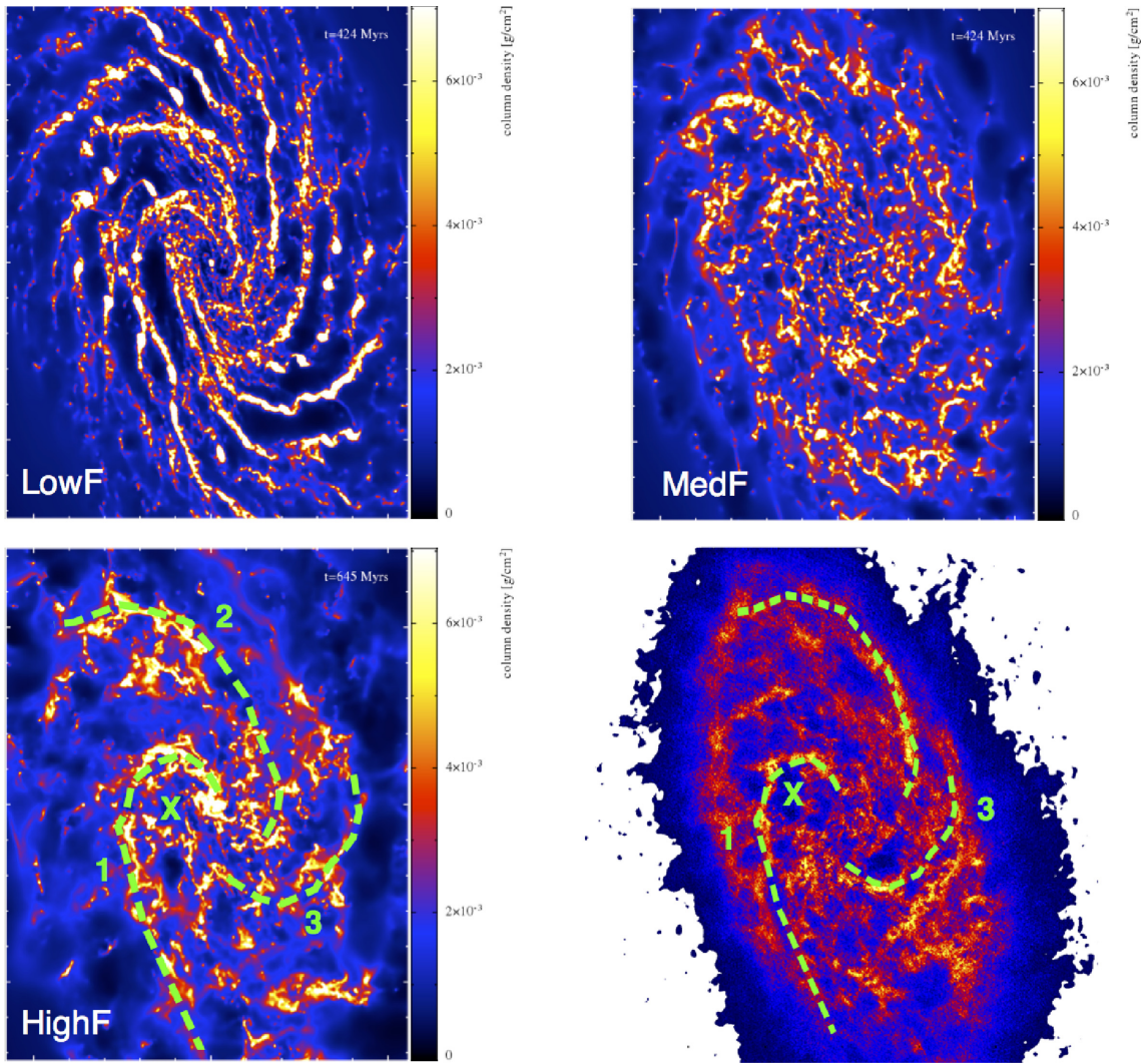
Figure 8. Column density images for different models presented in this paper compared with the actual M33 H I emission. All scales are linear, both for the observations and simulations. The top and bottom left panels show the models with different levels of feedback. The low feedback model (LowF) shows very strong spiral arms, and very bright dense clumps which are not seen in the actual M33. The medium feedback model shows less clear spiral arms compared to the actual M33. The best match by eye is the high feedback case. Here, the feedback is sufficient to create large holes or shells, which also appear to shape the gaseous arms and push the gas into a smaller number of arm features compared to the models with weaker feedback. For the models MedF and HighF, the time frames are shown when there is best agreement by eye with the real M33. Of all the models, only the HighF model shows particular differences in the structure (namely the appearance of large shells) with time such that the time of the snapshot is significant.
