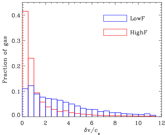
Figure 7. Fraction of gas exhibiting different values of \delta v/c_s where \delta v represents the change in velocity of the gas as it crosses a spiral arm, and thus \delta v/c_s > 1 represents shocks in the gas. The model with the low feedback efficiency exhibits a greater fraction of gas undergoing shocks, and thus the gas produces a stronger response to the underlying stellar structure, and clear spiral arms are seen. The model with the high feedback has less gas with large \delta v/c_s , and thus does not have such a strong response to the stellar structure.
