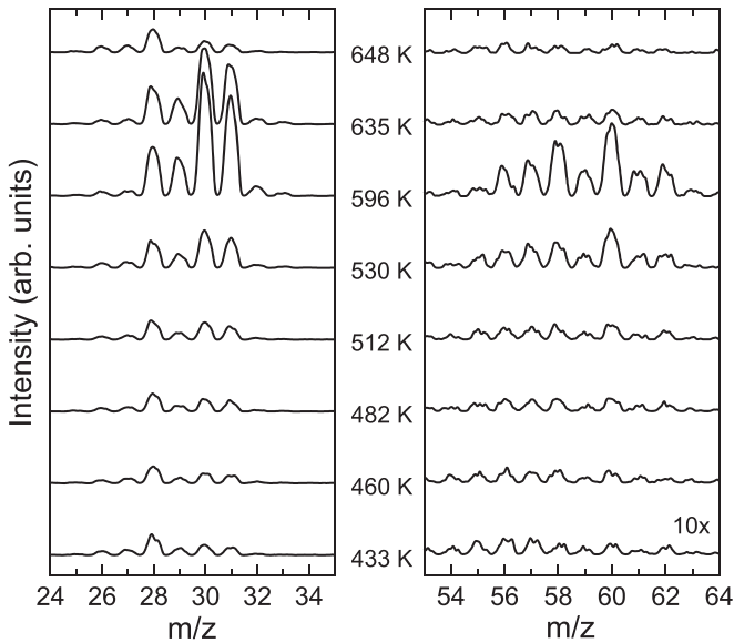
Figure 6. Thermal desorption of silane and disilane detected by the mass spectrometer during the annealing of the solid material synthesized following the \text{Si} + \text{H}_2 (1 sccm) reaction. The curves have been vertically shifted and the signal from m/z = 53 to m/z = 64 has been magnified 10 times for the sake of clarity.
