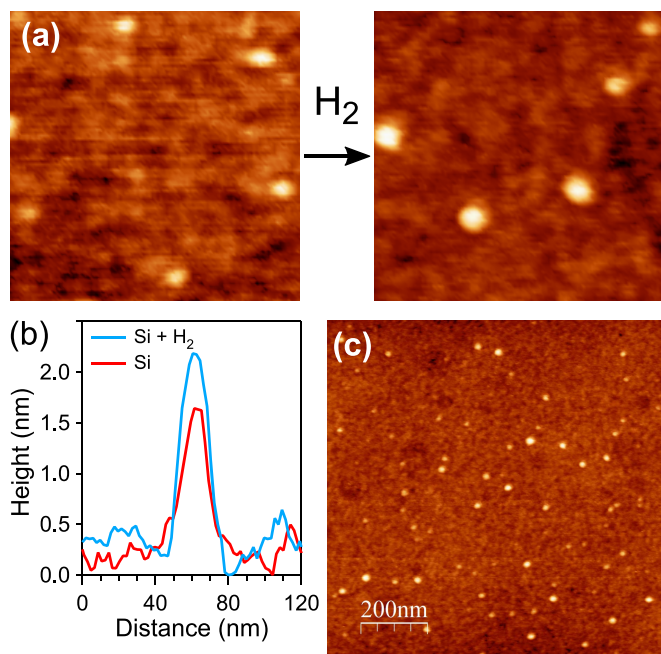
Figure 4. (a) AFM images ( 200 \times 200 \text{ nm}^2 ) of silicon nanoparticles: pure Si (left) and Si + H 2 (1 sccm) (right). (b) The height profiles of the nanoparticles show the increase in size after H 2 injection. (c) Lower magnification image of nanoparticles prepared following the reaction Si + H 2 (1 sccm).
