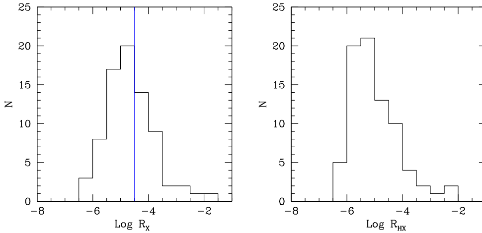
Figure 2. Left: X-ray radio loudness given by the ratio of the 1.4-GHz peak luminosity over the 2–10 keV luminosity. The blue line is the radio-loud versus radio-quiet limit set by Terashima & Wilson (2003). Right: hard X-ray radio loudness given by the ratio of the 1.4-GHz peak luminosity over the 20–100 keV luminosity.
