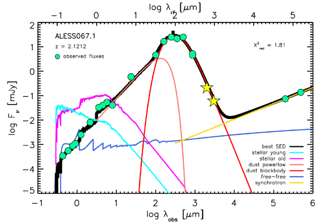
Figure A2. UV-radio best SED for ALESS067.1. Yellow filled stars stand for the ALMA B4 and B3 fluxes measured in this work (see B3 continuum contours in Fig. 3) and are not included in the SED fitting. Green filled circles represent the multiband available photometry. Error bars are omitted when comparable to symbol size.
