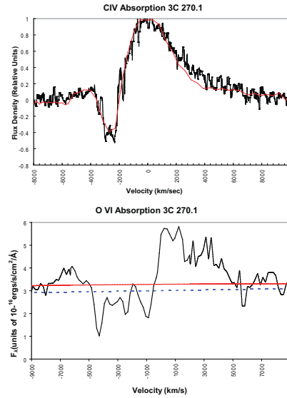
Figure 3. Ultraviolet absorption lines occur in the spectrum. The CIV line as measured by MMT is plotted in black in the top frame. The SDSS low resolution CIV spectrum is overlayed in red. The data is referenced to the estimated continuum level. The OVI absorption and emission line is plotted in the bottom frame. The solid red line is the fourth order polynomial fit and the dashed blue line is the power law fit to the continuum.
