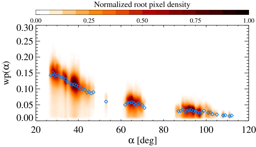
Fig. 7: wp(\alpha) distribution at 0.55 \mu m as a function of phase angle for \bar{\theta}_0 = 0^\circ . Blue diamonds represent the average values on 1^\circ phase angle bins.
