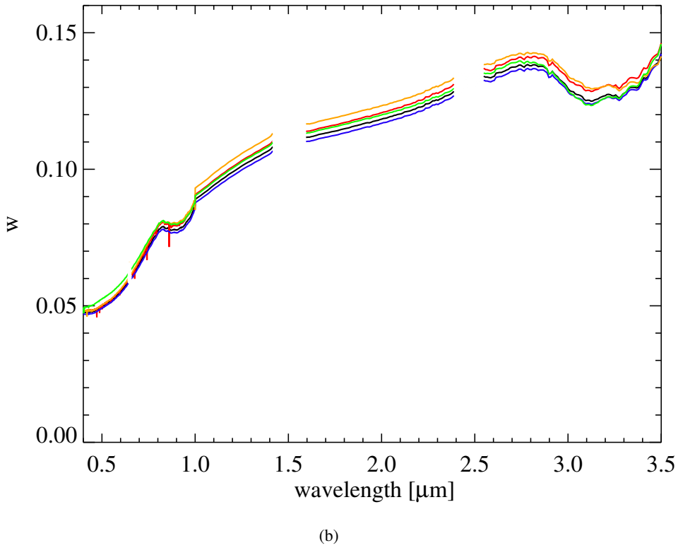
Fig. 21: Spectral variation of b (a) and w (b) for the four different macro-regions: head (red), neck (green), body (blue) and bottom (orange). The derived spectra from the global analysis are reported in black. The absorption common to all the spectra in the 0.8\text{--}1\text{ }\mu\text{m} is likely a residual artifact of calibration. Some abrupt oscillations of both w and b at certain wavelengths are due to degeneration in the fitting.
