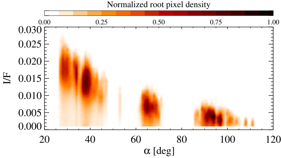
Fig. 6: a) I/F at 0.55 \mu m as a function of the phase angle: contour plot showing points density.
