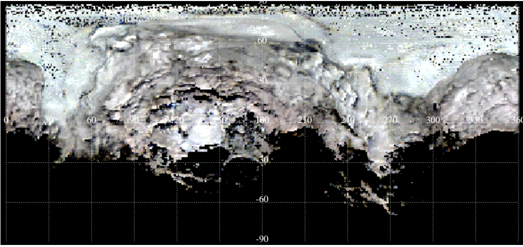
Fig. 20: Red ( 0.70\ \mu\text{m} ), green ( 0.55\ \mu\text{m} ) and blu ( 0.44\ \mu\text{m} ) SSA map.
