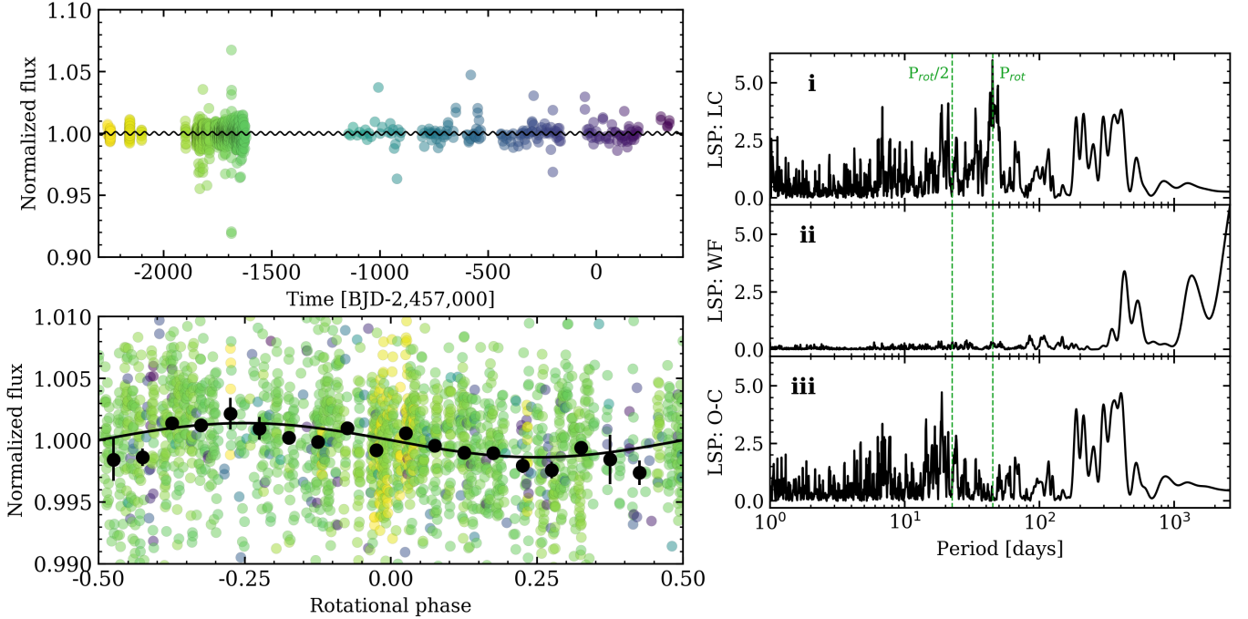
Figure 3. Measurement of the TOI-1235 photometric rotation period with MEarth-North. Upper left panel: the TOI-1235 differential light curve from archival MEarth-North photometry (October 2008–November 2015). Right panels: Lomb-Scargle periodograms of i) the detrended light curve, ii) the window function, and iii) the photometric residuals after removal of the optimized sinusoidal fit with P_{\text{rot}} = 44.7 days. Lower left panel: the light curve phase-folded to P_{\text{rot}} . Circular black markers represent the binned light curve while the solid black curve depicts the sinusoidal fit.
