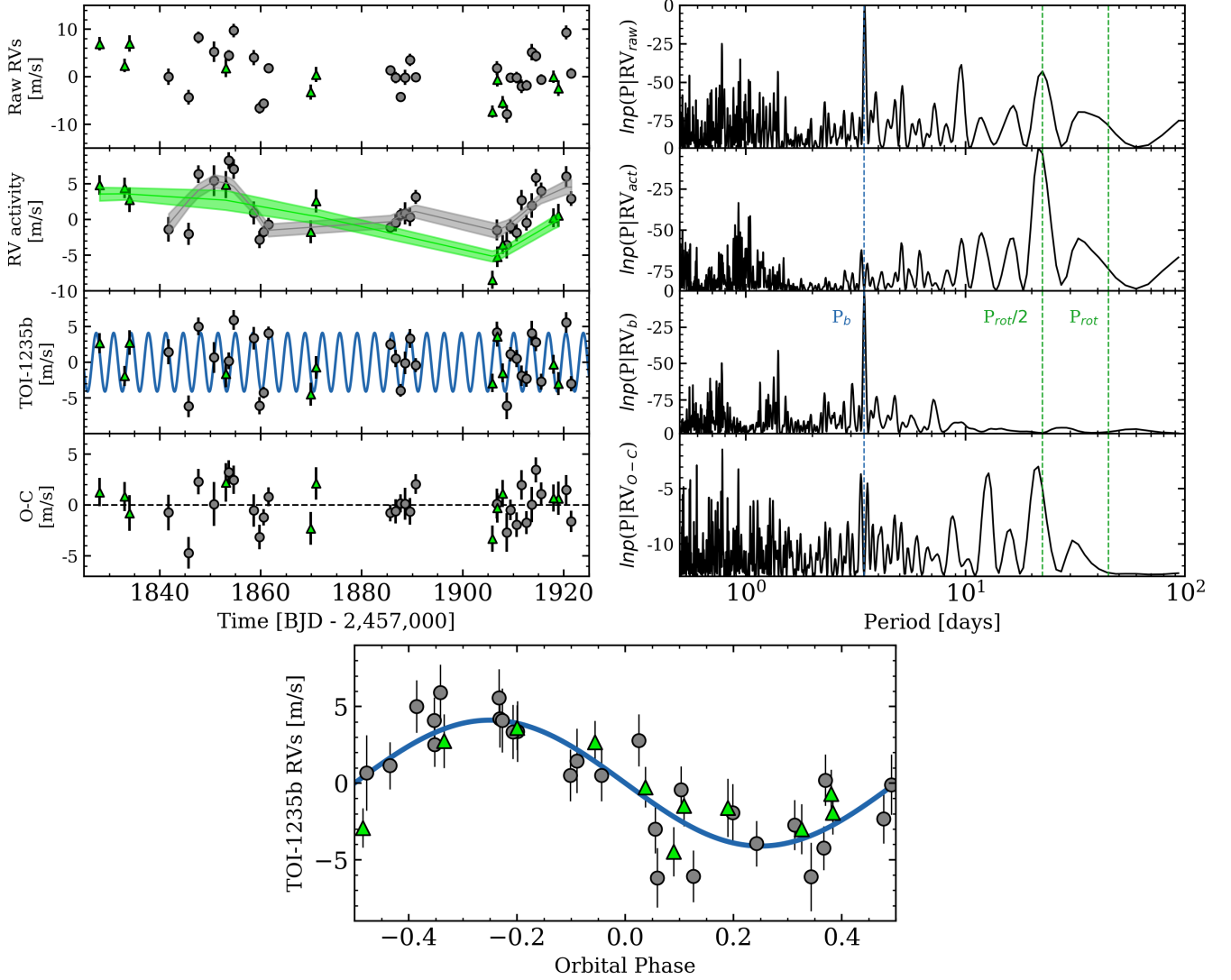
Figure 5. TOI-1235 RVs from HARPS-N ( gray circles ) and HIRES ( green triangles ). The data of each RV component and its corresponding model are depicted in the left column of the first four rows. Each component’s corresponding Bayesian generalized Lomb-Scargle periodogram is depicted in the adjacent right column with the vertical dashed lines highlighting the orbital period of TOI-1235 b ( P = 3.44 days), the stellar rotation period ( P_{\text{rot}} = 44.7 days), and its first harmonic ( P_{\text{rot}}/2 = 22.3 days). First row : the raw RVs. Second row : RV activity at P_{\text{rot}}/2 modeled as separate quasi-periodic GPs for each spectrograph. Third row : the Keplerian orbital solution for TOI-1235 b. Fourth row : the RV residuals. Bottom panel : the phase-folded RV signal from TOI-1235 b.
