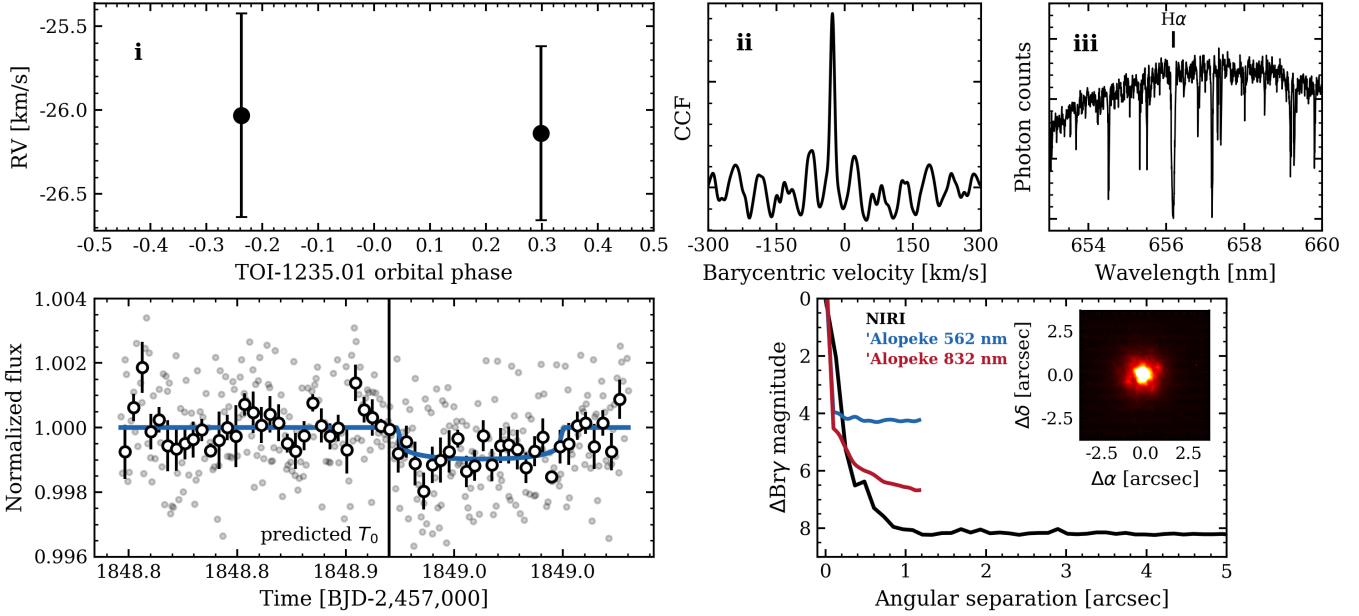
Figure 4. Summary of TFOP follow-up observations of TOI-1235 for planet validation purposes. Top row: results from TRES reconnaissance spectroscopy that i) show no RV variations thus ruling out a spectroscopic binary, ii) reveal a single-lined CCF with no rotational broadening, and iii) show H\alpha in absorption. Lower left panel: the ground-based transit light curve obtained with LCOGT showing that the expected transit event occurred on-target and arrived 63 minutes late relative to the SPOC-reported linear ephemeris represented by the black vertical line. Open circles depict the light curve in 5.5 minute bins. The blue curve depicts the optimized transit fit to the LCOGT photometry. Lower right panel: the 5\sigma contrast curves from Gemini/NIRI AO-imaging (black), ‘Alopeke 562 nm’ speckle imaging (blue), and ‘Alopeke 832 nm’ speckle imaging (red). The inset depicts the coadded image from Gemini/NIRI AO-imaging centered on TOI-1235.
