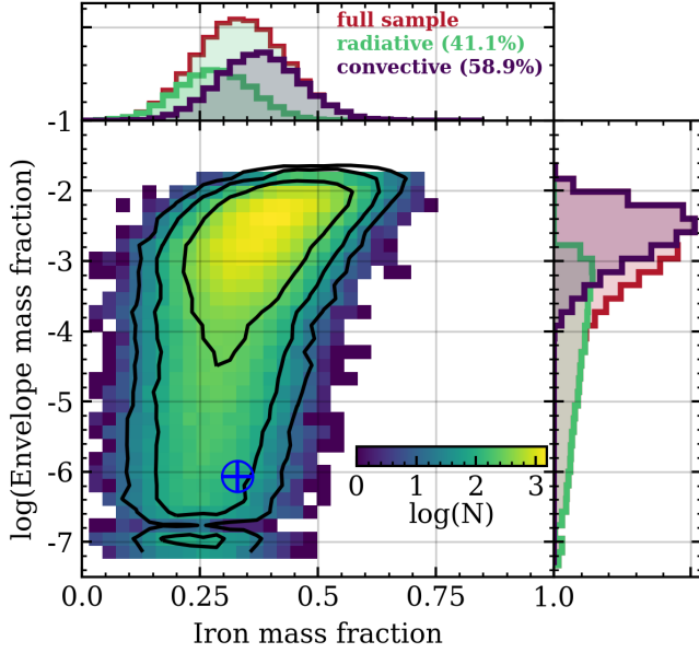
Figure 7. Joint distribution of TOI-1235 b’s iron mass and envelope mass fractions to be consistent with its measured mass and radius. The colormap represents the number of successful planet models given X_{\text{env}} and X_{\text{Fe}} while the contours highlight the 68, 95, and 99 percentiles. The top and right 1D histograms depict the marginalized distributions of X_{\text{Fe}} and \log_{10}(X_{\text{env}}) respectively for the full sample (red), plus the subset of realizations with a radiative atmospheres (green) and convective atmospheres (blue). The blue cross highlights the Earth.
