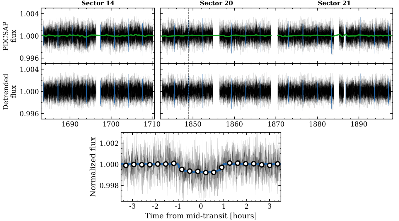
Figure 2. TESS light curve of TOI-1235 from sectors 14, 20, and 21. Upper row: the PDCSAP light curve following the removal of systematics via a linear combination of Cotrending Basis Vectors. The green curve depicts the mean GP model of residual temporally correlated noise (Sect. 4.1). The 3\sigma uncertainties on the mean GP model are smaller than the curve width. In-transit measurements are highlighted in blue throughout. The vertical dashed line highlights the epoch of the ground-based transit observation from LCOGT, which confirms the transit event on-target (Sect. 3.4). Lower row: the detrended PDCSAP light curve. Bottom panel: the phase-folded transit light curve of TOI-1235 b from 22 individual transit events. The maximum a-posteriori transit model is depicted by the blue curve while the white markers depict the binned photometry.
