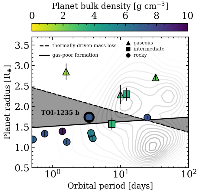
Figure 8. Period-radius diagram for small planets orbiting M dwarfs with precise RV masses including TOI-1235 b ( bold circle ). The dashed and solid lines depict the locations of the radius valley around low mass stars from model predictions of thermally-driven atmospheric mass loss and from gas-poor terrestrial planet formation respectively. The shaded regions highlight where the predictions of planetary bulk compositions are discrepant between the two models. Contours represent the planetary occurrence rates around low mass stars (CM19). Planet marker shapes depict the planet’s compositional disposition as either rocky ( circles ), gaseous ( triangles ), or intermediate ( squares ). Marker colors indicate the planet’s bulk density.
