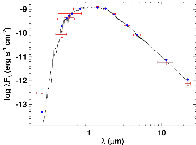
Figure 1. The spectral energy distribution of TOI-1235. Red markers depict the photometric measurements with horizontal errorbars depicting the effective width of each passband. Black curve depicts the most likely stellar atmosphere model with T_{\text{eff}} = 3950 K. Blue circles depict the model fluxes over each passband.
