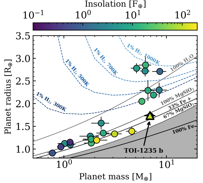
Figure 6. Mass-radius diagram for small planets orbiting M dwarfs including TOI-1235 b (triangle marker). Errorbars on the TOI-1235 b mass and radius are smaller than the marker, which lies directly on top of LHS 1140 b in this space. The solid curves depict internal structure models with mass fractions of 100% water, 100% silicate rock, 33% iron plus 67% rock (i.e. Earth-like), and 100% iron (Zeng & Sasselov 2013). The dashed curves depict models of Earth-like cores hosting \text{H}_2 envelopes with 1% envelope mass fractions at various equilibrium temperatures (Zeng et al. 2019). The shaded region bounded by the dotted curve highlights the forbidden region according to models of maximum collisional mantle stripping by giant impacts (Marcus et al. 2010).
