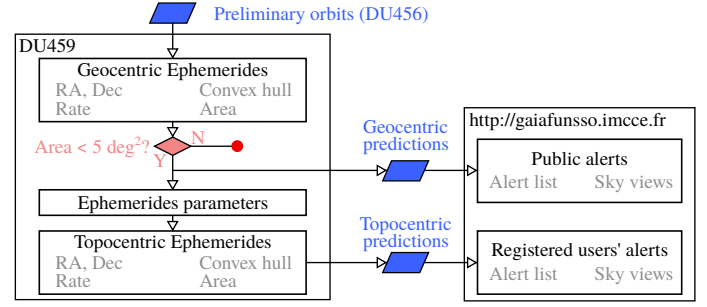
Fig. 4. Simplified workflow of alert processing and diffusion. Alerts are selected based on geocentric ephemerides. For each alert below the area threshold, topocentric ephemerides are computed for each observatory in the system. All ephemerides are stored in a database that is used by the Web pages.
