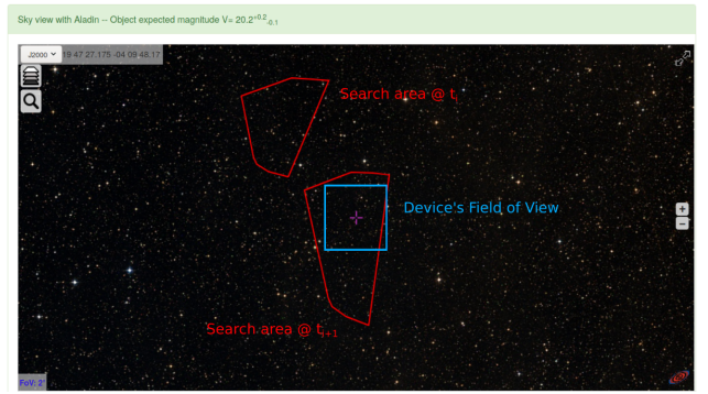
Fig. 5. Example of the sky view of alerts with AladinLite. The red polygons correspond to the convex hull of the cloud of predicted positions at different dates, and the blue square represents the field of view of the device defined by the user (only available upon registration).
