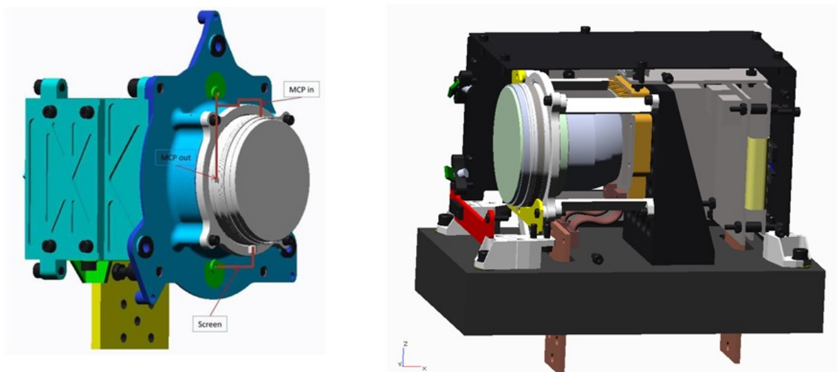
Figure 3. CAD derived views of the Metis (left panel) and the EUI (right panel) Lyman-alpha cameras showing the mounting of the intensifiers.
