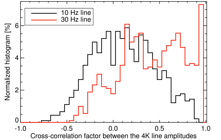
Figure 7. Normalized histograms of the correlation coefficients of the 10 and 30 Hz 4-K line amplitudes. The amplitude is computed per ring and per bolometer from the two coefficients (sine and cosine) of a given line. For each pair of distinct bolometers (from 100 to 353 GHz), a correlation coefficient is computed between the two amplitudes during the mission. The black normalized histogram shows the 10 Hz line correlation coefficients of the 903 ( = 43 \times 42/2 ) pairs. The red curve shows the 30 Hz line histogram. The 30 Hz line is clearly correlated between different bolometers. This is the only line that shows a significant correlation.
