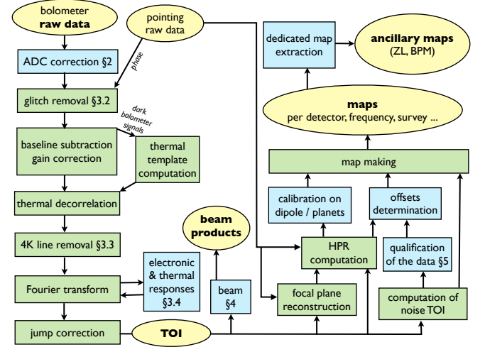
Figure 1. Schematic of the HFI pipeline. The left part of the schematic involves TOI and beams (this paper), while the upper-right part represents the map making steps (Paper 2). Ancillary maps are composed of zodiacal light templates (ZL) and polarization band-pass mismatch (BPM) maps. ADC = analogue-to-digital converter (see Sect. 2). HPR = HealPix ring (see Paper 2). “Beam products” refers to beam transfer functions, B_\ell . Blue: changes in this release with section numbers corresponding to this paper. Yellow: released data products.
