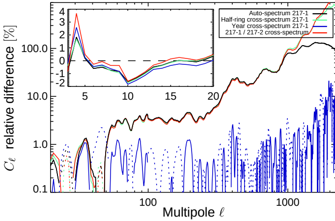
Figure 20. Relative differences of the C_\ell , computed on 60 % of the sky, using data processed with and without the thermal decorrelation. Note that the zero-level has been recomputed in all cases to allow the comparison to be made. The amplitudes of the negative values are shown by dotted lines.
