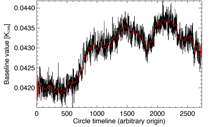
Figure B.2. The baseline for each circle for bolometer 100-3b and the first scan of Mars (black line), and smoothed with a 40-circle sliding window (red line).
