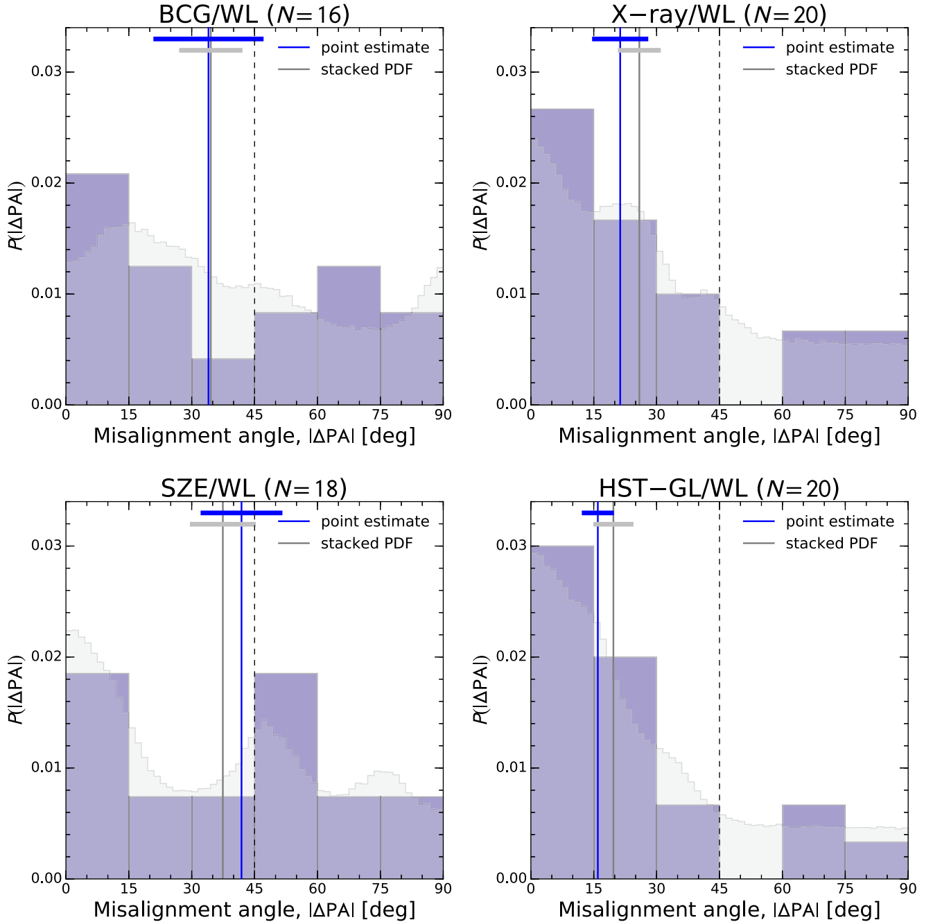
Figure 6. Histogram of the absolute misalignment angles |\Delta PA| between the BCG/WL (upper left), X-ray/WL (upper right), SZE/WL (lower left), and HST -GL/WL (lower right) major axes. In each panel, the blue and gray shaded histograms show the distributions constructed from posterior point estimates ( C_{BI} ) and from the stacked composite PDF, respectively. For each histogram, the median value of the distribution is indicated by a vertical line, and its 1\sigma error by a thick horizontal line. In the absence of any alignment, the expected median value is 45^\circ (vertical dashed line).
