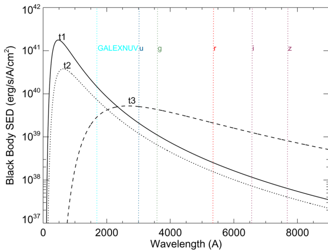
Figure 2. SEDs at three characteristic times for a standard NS10 model of a RSG progenitor with 500 R_{\odot} , 15 M_{\odot} and 1 foe. The mean wavelengths of filters NUV GALEX and Sloan griz are shown.
