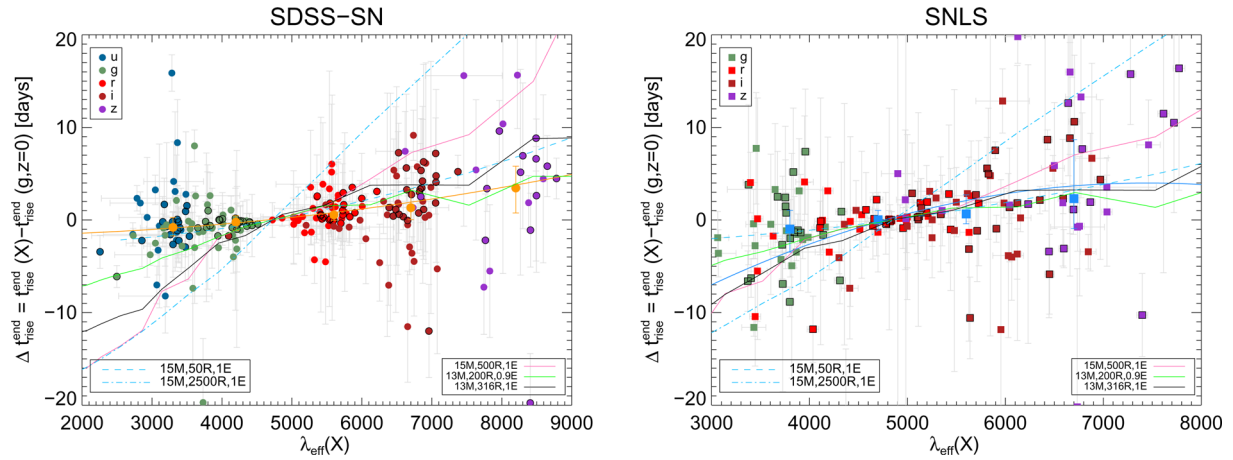
Figure 11. Difference in rise-times, \Delta t_{\text{rise}}^{\text{end}} , respect to an interpolated rise-time at g -band rest frame ( \lambda_{\text{eff}} = 4722 \text{ \AA} ) for the SDSS-SN (left) and SNLS (right) samples. Points with black contours are the golden samples and larger symbols are the median values at characteristic wavelengths. The best second-order polynomial fit is shown as a solid line (orange for SDSS-SN and blue for SNLS). Overplotted are representative analytical models from RW10 for extreme radii of 50 R_{\odot} (blue dotted) and 2500 R_{\odot} (blue dashed), and hydrodynamical models from T09 for a standard 500 R_{\odot} (pink), a more compact 200 R_{\odot} (green) and a dense progenitor with 316 R_{\odot} (black).
