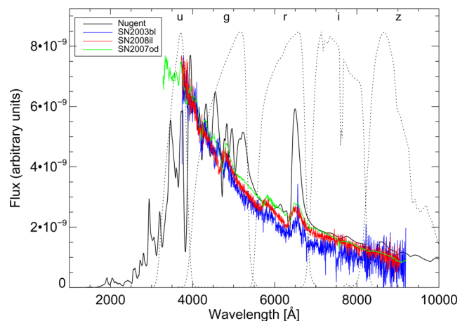
Figure B1. SN II spectral template by Nugent (black) compared to observed rest-frame MW-corrected SN II spectra of SN 2003bl at \sim 2 d after explosion (blue), SN 2008il at \sim 3 d after explosion (red) and SN 2007od at 6 d after explosion (green). Broad-band SDSS filters are shown as dashed lines.
