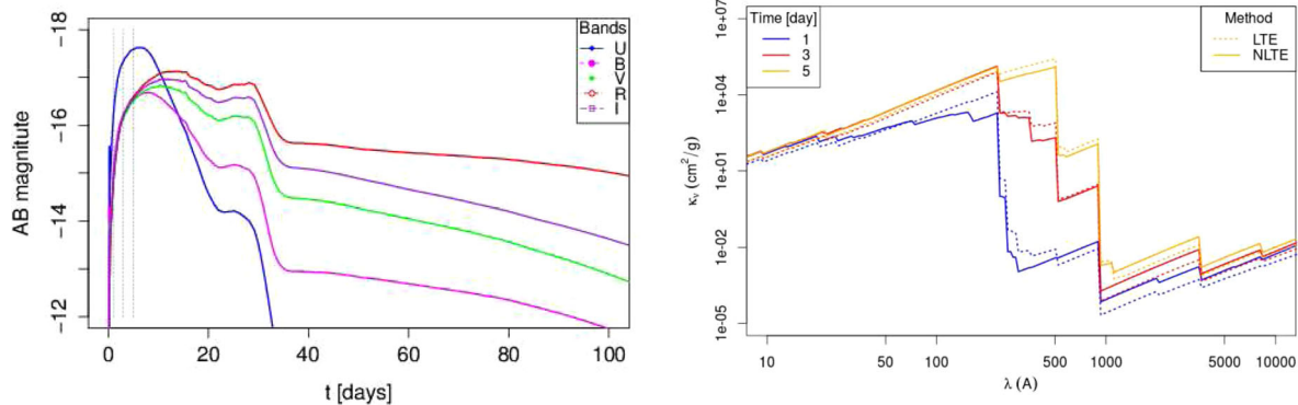
Figure A1. Left: UBVRI light curves of SN models. The dotted lines show three time points t = 1, 3, 5 d used for the analysis of the role of the non-LTE effects. Right: the wavelength-dependent expansion opacities, \kappa , are plotted at time moments t = 1, 3, 5 d. The opacity is calculated using both LTE (dotted) and non-LTE (solid) assumptions to demonstrate the reliability of the LTE approach.
