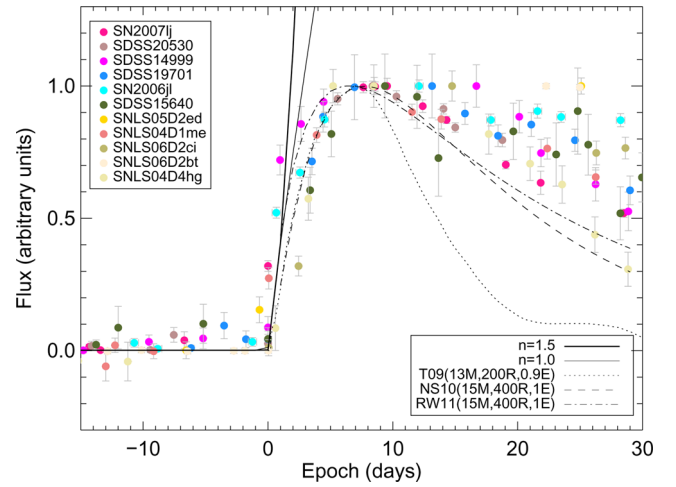
Figure 12. Aggregate light curves of 11 SNe II from the SDSS-SN and SNLS that have fitted power-law rise-times between 6.5 and 7.5 d. The solid lines show power laws of n = 1.5 (thick) and 1.0 (thin). The dotted line is the hydrodynamical model by T09 with R = 200 R_{\odot} (with n = 1.3 ), while the dashed and dot-dashed are the analytical models by NS10 and RW11 with R = 400 R_{\odot} (with n = 1.0 and 0.8 , respectively).
