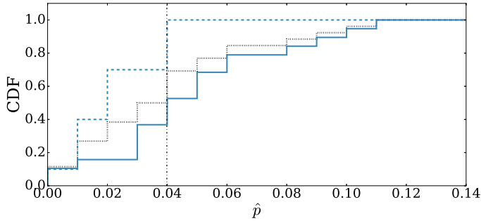
Fig. 2. J1505+0326: Distribution of the debiased polarisation fraction \hat{p} . The dot-dashed vertical line marks the median of the distribution. The blue dashed line shows the distribution of \hat{p} during the non-rotating phases and the solid line shows this during the rotating phases. The black dotted line corresponds to all the measurements.
