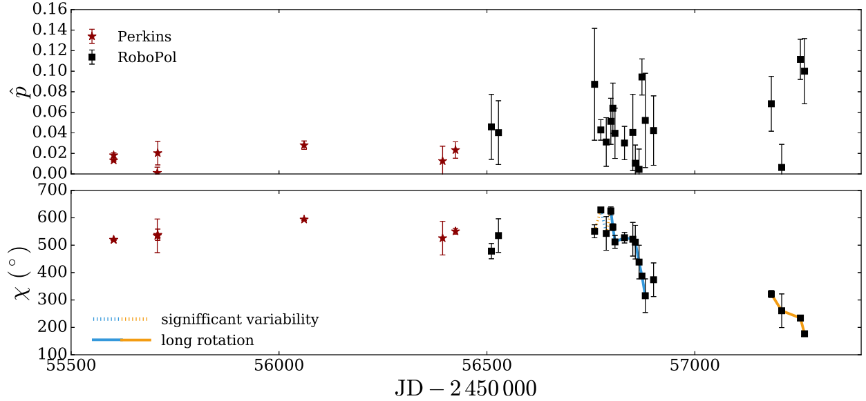
Fig. 1. J1505+0326: Debiased polarisation fraction p and adjusted EVPA ( \chi ) as a function of time. The coloured lines mark periods of significant monotonous (within the uncertainties) EVPA evolution. Solid lines mark periods of long rotations (i.e. at least three sequential data points and an angle larger than 90^\circ ). Blue and orange connecting lines are used alternately for clarity.
