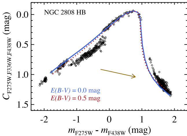
Figure 3. Observed HB distribution of NGC 2808 (black points) in the CCP that highlights its HB discontinuities. The extinction vector for a 12,000 K BHB star is shown (brown arrow). Strictly speaking, the extinction vector in this plane is SED dependent. However, for the purposes of empirical comparisons to the other clusters in our sample, one can assume an SED-independent extinction vector and simply shift the HB distribution of any cluster to align with that of NGC 2808, using the C_{\text{peak}} as a fiducial. We demonstrate the accuracy of this approach by shifting a theoretical ZAHB distribution to align with the observations at the C_{\text{peak}} , using two different extinction assumptions. In one case, no foreground reddening was applied before the alignment (solid blue curve), and in the other, significant SED-dependent reddening was applied before the alignment (dotted red curve), but the distinction between the two curves is small. The deviation of the observed BHB below the ZAHB curves at -1.2 < (m_{F275W} - m_{F438W}) < -0.2 mag is due to radiative levitation blueward of the G-jump. The stars falling to the blue of the ZAHB curves, at (m_{F275W} - m_{F438W}) < -1.8 mag, are blue-hook stars, with effective temperatures hotter than the canonical end of the EHB.
