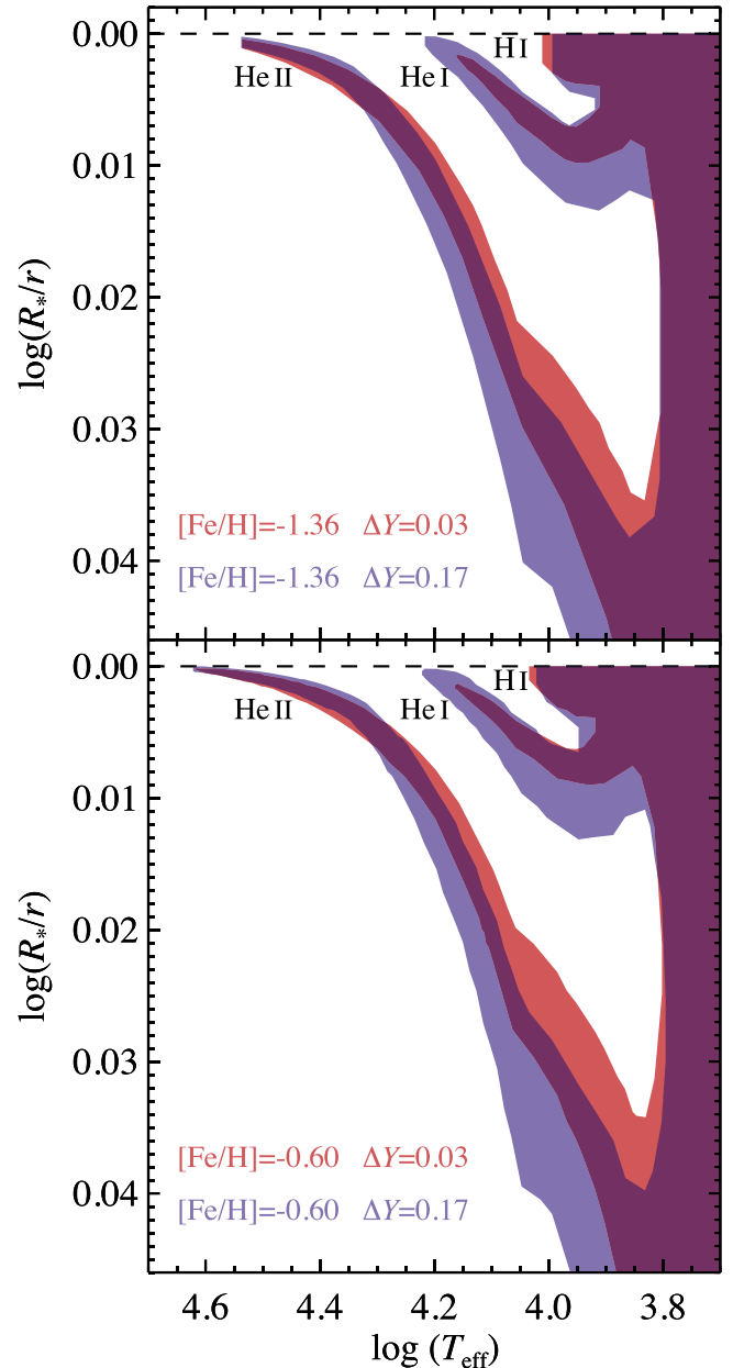
Figure 9. The location of the convection zones (shading) in ZAHB stars as a function of effective temperature, relative to the stellar surface (dashed line), assuming the metallicity of NGC 2808 (top panel) and NGC 6388 (bottom panel). When the He abundance is increased from \Delta Y = 0.03 (red shading) to \Delta Y = 0.17 (blue shading), the transition in the He I convective zone shifts to higher effective temperature by \sim 2000 K, and the He I convective zone moves closer to the surface. If the G-jump is normally associated with the He I convective zone, this temperature shift at high Y may explain the bluer G-jump in NGC 6388 and NGC 6441. If the G-jump is normally associated with the H convective zone, the surface encroachment of the He I convective zone at high Y may also explain the bluer G-jump in NGC 6388 and NGC 6441. Note that evolutionary effects, turbulence, and mass loss complicate this interpretation; these models only serve to provide possible explanations for the observed G-jump behavior in a qualitative sense. Similarly, if the M-jump is associated with the He II convective zone, the observed consistency of the M-jump temperature (even in NGC 6388 and NGC 6441) might be due to the insensitivity of the He II convective zone to Y .
