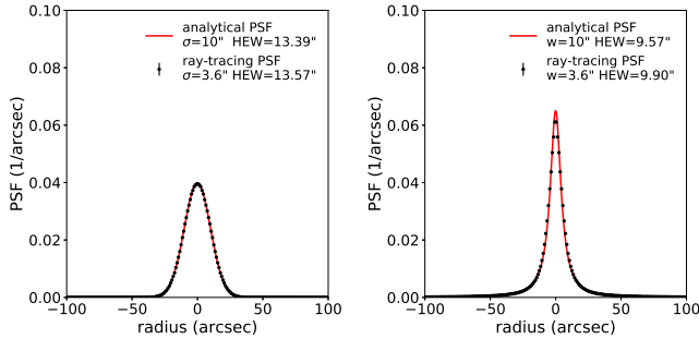
FIG. 4. PSF simulation obtained from ray-tracing model in Geant4 and analytical formula, with Gaussian shape (left) and Lorentzian shape (right) slope perturbation function.
