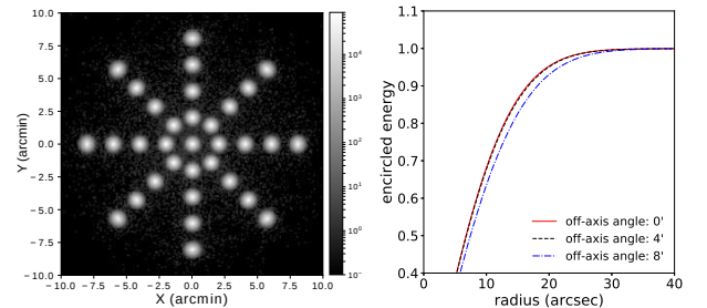
FIG. 7. PSF at different off-axis (ranging from 0' to 8' ) and azimuthal angles (every 45^\circ ) within FOV for 1 keV photons (left). 10^6 photons are simulated for each condition. EEF of the eXTP mirror at different off-axis angles for 1 keV photons (right).
