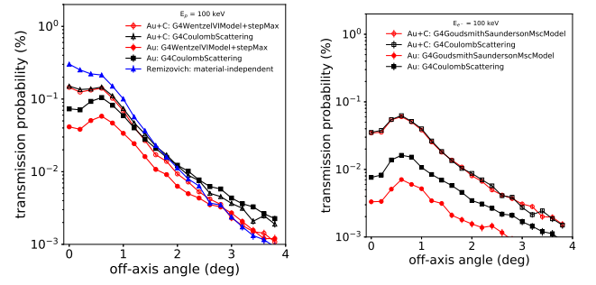
FIG. 18. The transmission probability of protons (left) and electrons (right) respectively, by using different selective layer materials.
