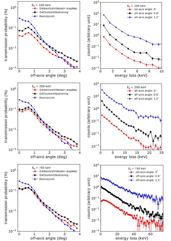
FIG. 16. The proton response of mirror at different incident energies, including the transmission probability and energy loss distribution. The energy loss distribution at different off-axis angles is scaled for better visibility.
