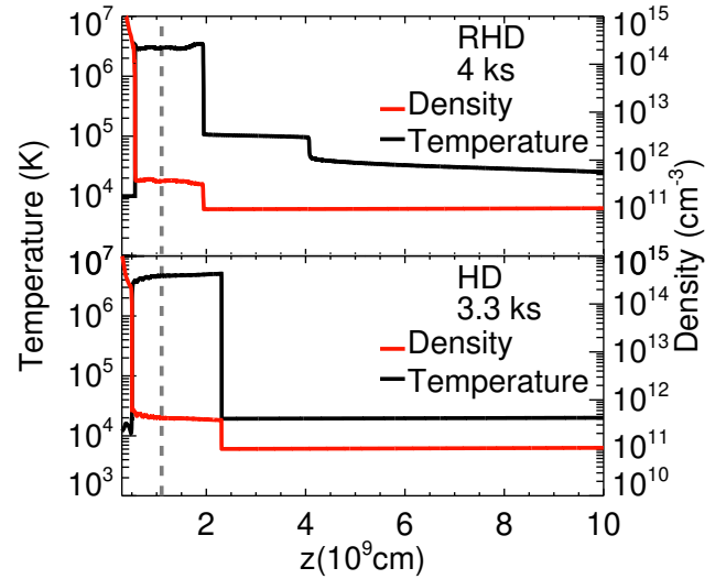
Fig. 4. Temperature (black line) and density (red line) profiles for runs RHD (top panel) and HD (bottom panel), during one of the expanding phases. The gray dotted line marks the initial position of the chromosphere.
