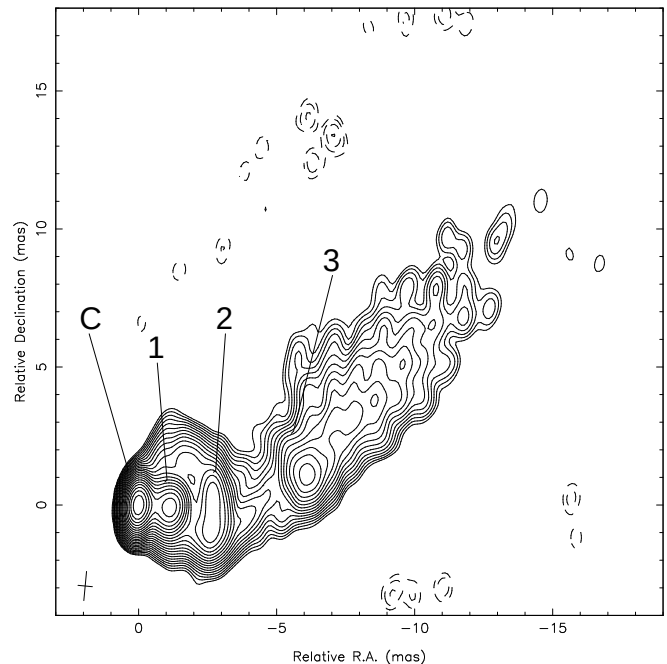
FIG. 9.— VLBI image of 3C 454.3 at 15 GHz on 2007 August 9 (MJD 54321). The peak flux density is 2.8 \text{ Jy beam}^{-1} and contours are traced at \pm(1, \sqrt{2}, 2, \dots) \times 1.0 \text{ mJy beam}^{-1} . The cross in the bottom left corner shows the beam FWHM, which is 1.07 \times 0.52 \text{ mas} at -5.4 \text{ deg} .
