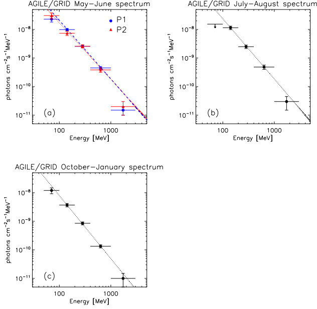
FIG. 2.— Panel (a): AGILE/GRID average \gamma -ray spectrum for periods P1 and P2. The blue-dashed and the red-dotted lines represent the best-fit power law models for P1 and P2, respectively. Panel (b) and Panel (c) show the average \gamma -ray spectra during the periods July–August 2008 and October 2008 - January 2009, respectively. In the three panels only three energy bins were considered for the spectral fitting: 100 < E < 200 MeV, 200 < E < 400 MeV, 400 < E < 1000 MeV (see text for details). [See the electronic edition of the Journal for a color version of this figure.]
