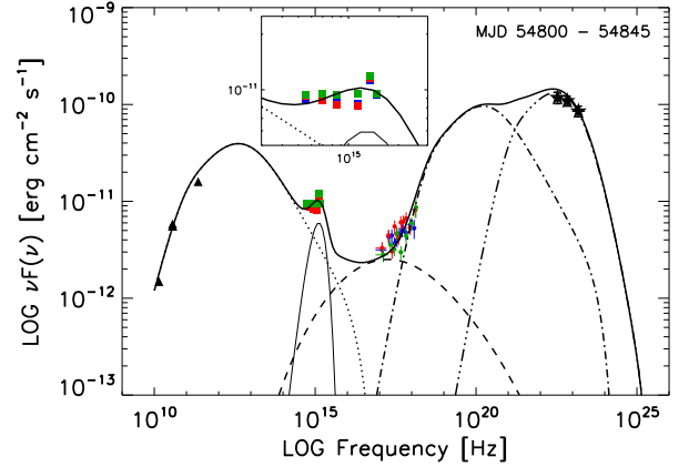
FIG. 19.— 3C 454.3 SED during the period MJD 54800–54845. Black triangles, multicolor squares, circles, and black stars represent radio, Swift /UVOT, Swift /XRT, and AGILE/GRID data, respectively. UV and X-ray data are de-reddened and corrected for Galactic extinction. The thin solid, dotted, dashed, dot-dashed, and the triple-dot-dashed, represent the accretion disk blackbody, the synchrotron, the SSC, the external Compton on the disk, and the external Compton on the BLR radiation, respectively. The thick solid line represent the sum of all the individual components. The insert shows the portion of the SED dominated by the contribution of the disk blackbody radiation.
