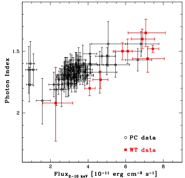
FIG. 4.— Swift/XRT photon index as a function of the 2–10 keV flux. Red squares and black circles mark the Swift/XRT windowed timing (WT) and photon counting (PC) data, respectively.
