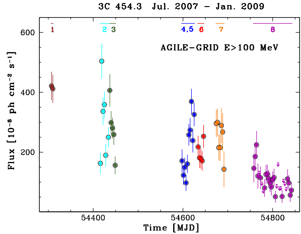
FIG. 11.— AGILE/GRID light curve at \approx 3 -day resolution for E > 100 MeV in units of 10^{-8} photons \text{cm}^{-2} \text{s}^{-1} . Different colors correspond to different observing campaigns, as described in Table 1.
