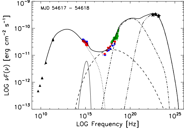
FIG. 17.— 3C 454.3 SED centered on MJD 54617–54618. Black triangles, red (blue) squares, red (blue) circles, green circles, and black stars represent radio, MJD 54617 (54618) Swift /UVOT, MJD 54617 (54618) Swift /XRT, RXTE/PCA, and AGILE/GRID data, respectively. UV and X-ray data are de-reddened and corrected for Galactic extinction. The thin solid, dotted, dashed, dot-dashed, and the triple-dot-dashed, represent the accretion disk blackbody, the synchrotron, the SSC, the external Compton on the disk, and the external Compton on the BLR radiation, respectively. The thick solid line represent the sum of all the individual components.
