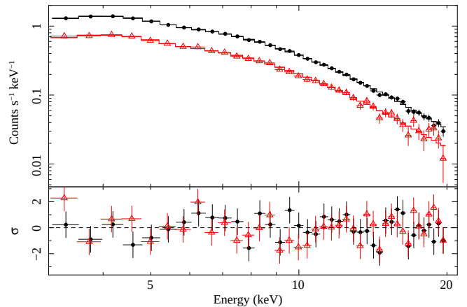
FIG. 6.— RXTE/ PCA average spectra for both periods, July 2007 (black points), and May-June 2008 (red triangles), respectively. [See the electronic edition of the Journal for a color version of this figure.]
