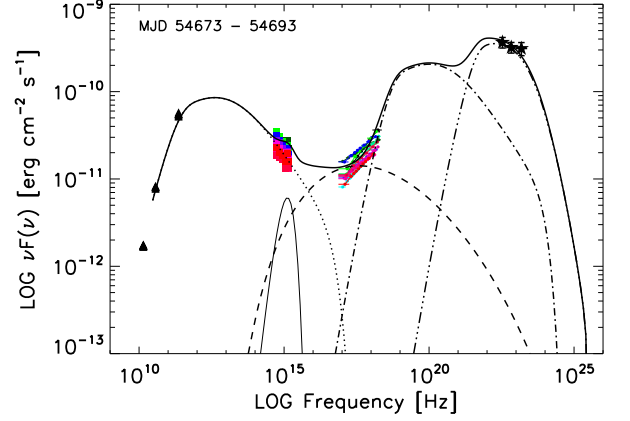
FIG. 18.— 3C 454.3 SED during the period MJD 54673–54693. Black triangles, multicolor squares, circles, and black stars represent radio, Swift /UVOT, Swift /XRT, and AGILE/GRID data, respectively. UV and X-ray data are de-reddened and corrected for Galactic extinction. The thin solid, dotted, dashed, dot-dashed, and the triple-dot-dashed, represent the accretion disk blackbody, the synchrotron, the SSC, the external Compton on the disk, and the external Compton on the BLR radiation, respectively. The thick solid line represent the sum of all the individual components.
