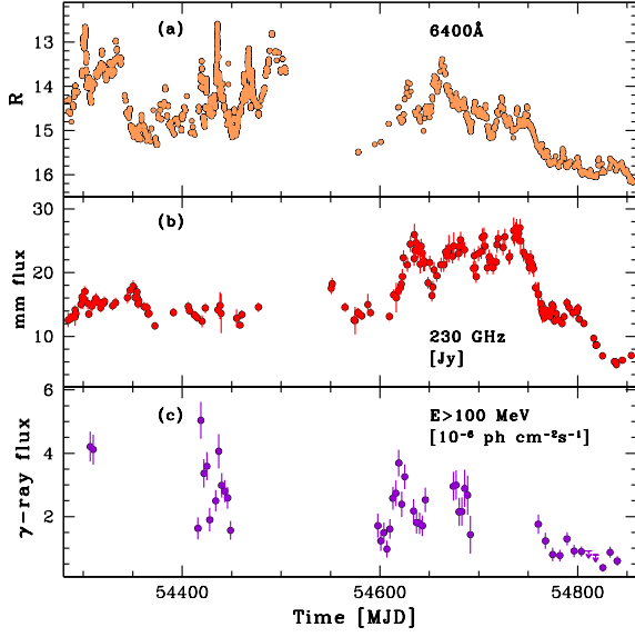
FIG. 13.— Comparison between the light curves in different bands. Panel (a), (b), and (c) show the light curves in the optical, millimeter, and \gamma -ray energy bands, respectively.
