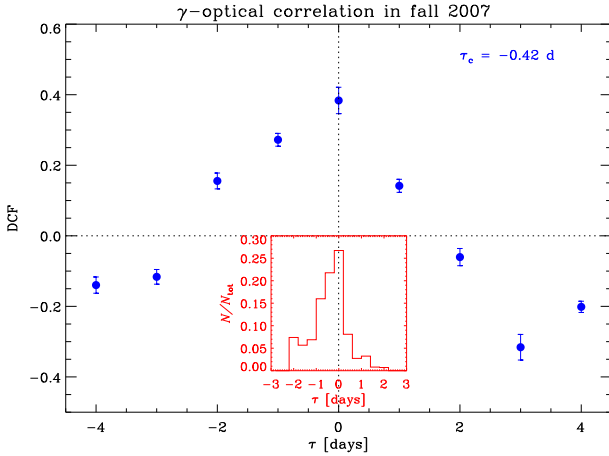
FIG. 14.— Discrete correlation function between the \gamma -ray and optical fluxes during the “fall 2007” period. The uncertainty in the time-lag can be computed according to the FR/FSS method. The inset shows the resulting centroid distribution (see text for details).
