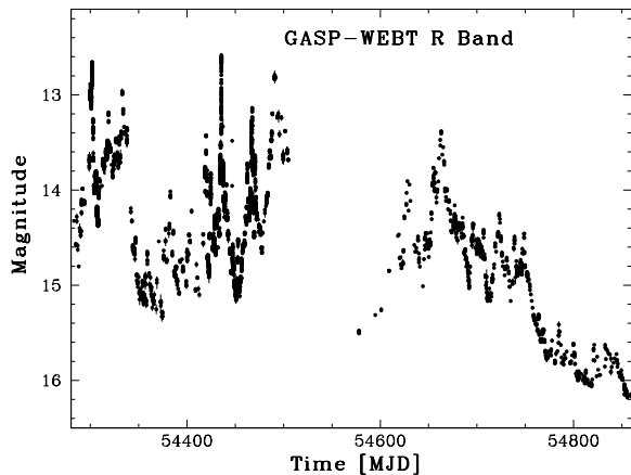
FIG. 7.— GASP-WEBT light curve in the R optical band in the 2007–2008 and 2008–2009 observing seasons.
