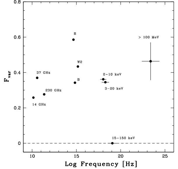
FIG. 15.— Fractional rms variability amplitude as a function of frequency.
