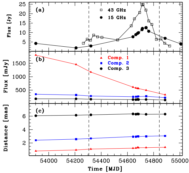
FIG. 10.— Panel (a): radio core flux density at 15 GHz (filled circles) and at 43 GHz (open squares), respectively. Panel (b): radio components flux density at 15 GHz. Panel (c): radio components motion at 15 GHz. The vertical dashed lines represent the start (2007 July 24) and the stop (2009 January 12) of all AGILE observations, respectively.
