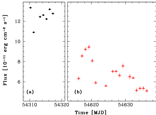
FIG. 5.— Panel (a) and (b) show the RXTE/ PCA light curve in the energy band 3–20 keV during the periods 2007 July 29 - August 5 (black points) and 2008 May 30 - June 19 (red triangles), respectively. [See the electronic edition of the Journal for a color version of this figure.]
