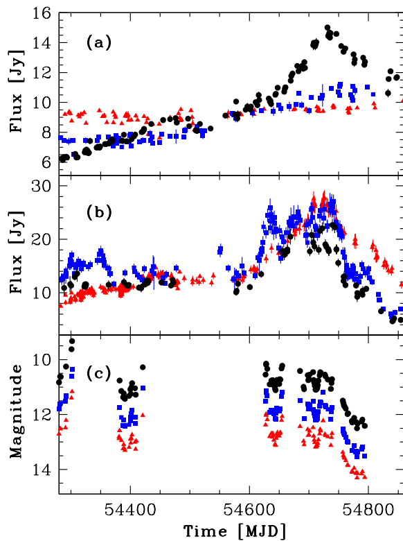
FIG. 8.— Panel (a) : low-frequency radio data. Red triangles, blue squares and black circles represent the radio flux at 5, 8, and 14.5 GHz, respectively. Panel (b) : high-frequency radio data. Red triangles, blue squares, and black circles represent the radio flux at 37, 230, and 345 GHz, respectively. Panel (c) : near-IR data. Red triangles, blue squares, and black circles, represent the J , H , and K bands, respectively [See the electronic edition of the Journal for a color version of this figure.]
