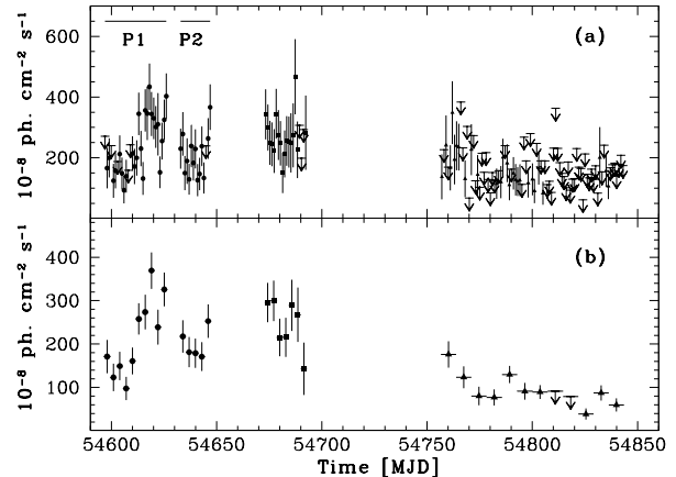
FIG. 1.— Panel (a): AGILE/GRID \gamma -ray light curve at \approx 1 -day resolution for E > 100 MeV in units of 10^{-8} photons \text{cm}^{-2} \text{s}^{-1} during the period May 2008 - January 2009. The downward arrows represent 2\sigma upper-limits. Panel (b): the same as in panel (a), but with a time bin of three (filled circles and squares), and seven (filled triangles) days, respectively.
