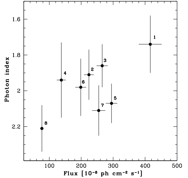
FIG. 16.— AGILE/GRID photon index as a function of the \gamma -ray flux above 100 MeV. Number beside each points represents the epochs listed in Table 1.
