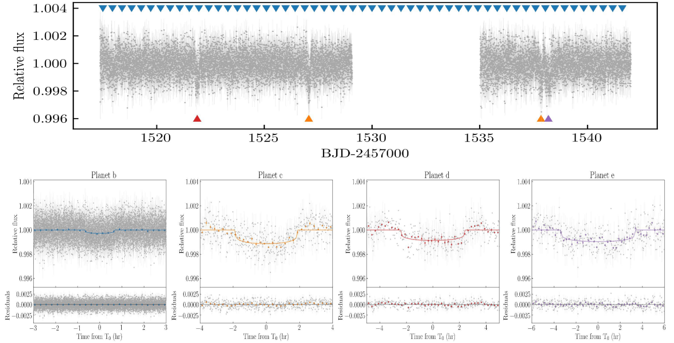
Figure 6. Top panel: 2-min cadence flattened light curve of TOI-561. The transits of planet b ( P \sim 0.45 d), c ( P \sim 10.8 d), d ( P \sim 25.6 d), e ( P \sim 77.2 d) are highlighted with blue, orange, red, and purple triangles, respectively. Bottom panels: TOI-561 phase-folded 2-min light curves over the best-fitting models (solid lines) for the four planets. The light-curve residuals are shown in the bottom panels.
