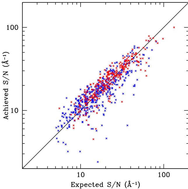
Figure 5. Measured S/N per \text{\AA} (averaged over 8030 \text{ \AA} – 8270 \text{ \AA} ) for the first year of data vs. the expected S/N, based on i^+ band magnitude and galaxy size, calculated in preparation of the survey. Blue crosses indicate star-forming galaxies, red crosses quiescent galaxies. The general agreement implies that our predictions were accurate and that the data quality is as expected, if not slightly better. The scatter can be explained by variations in radial surface brightness profiles, axis ratios, position angles, and observing conditions.
