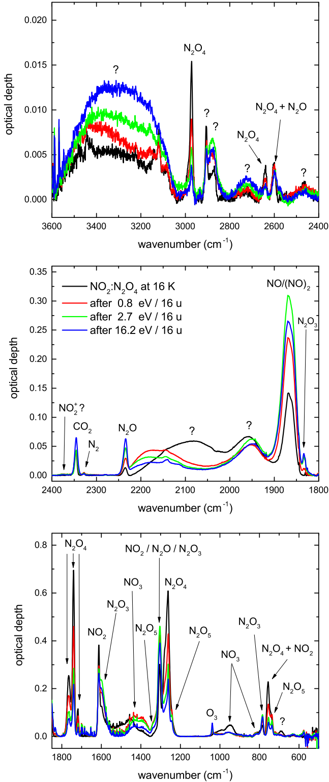
Figure 6. IR spectra of the icy mixture \text{NO}_2:\text{N}_2\text{O}_4 deposited at 16 K and after three irradiations (see label). For the sake of clarity three different spectral regions are shown, with optimized y-scale. Unidentified bands are indicated with a question mark.
