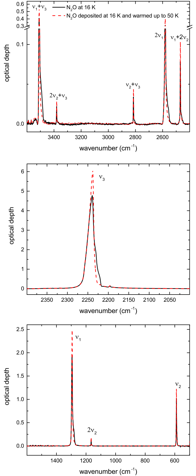
Figure 1. IR spectra of \text{N}_2\text{O} ices (i) grown at 16 K and (ii) grown at 16 K and warmed up to 50 K.
