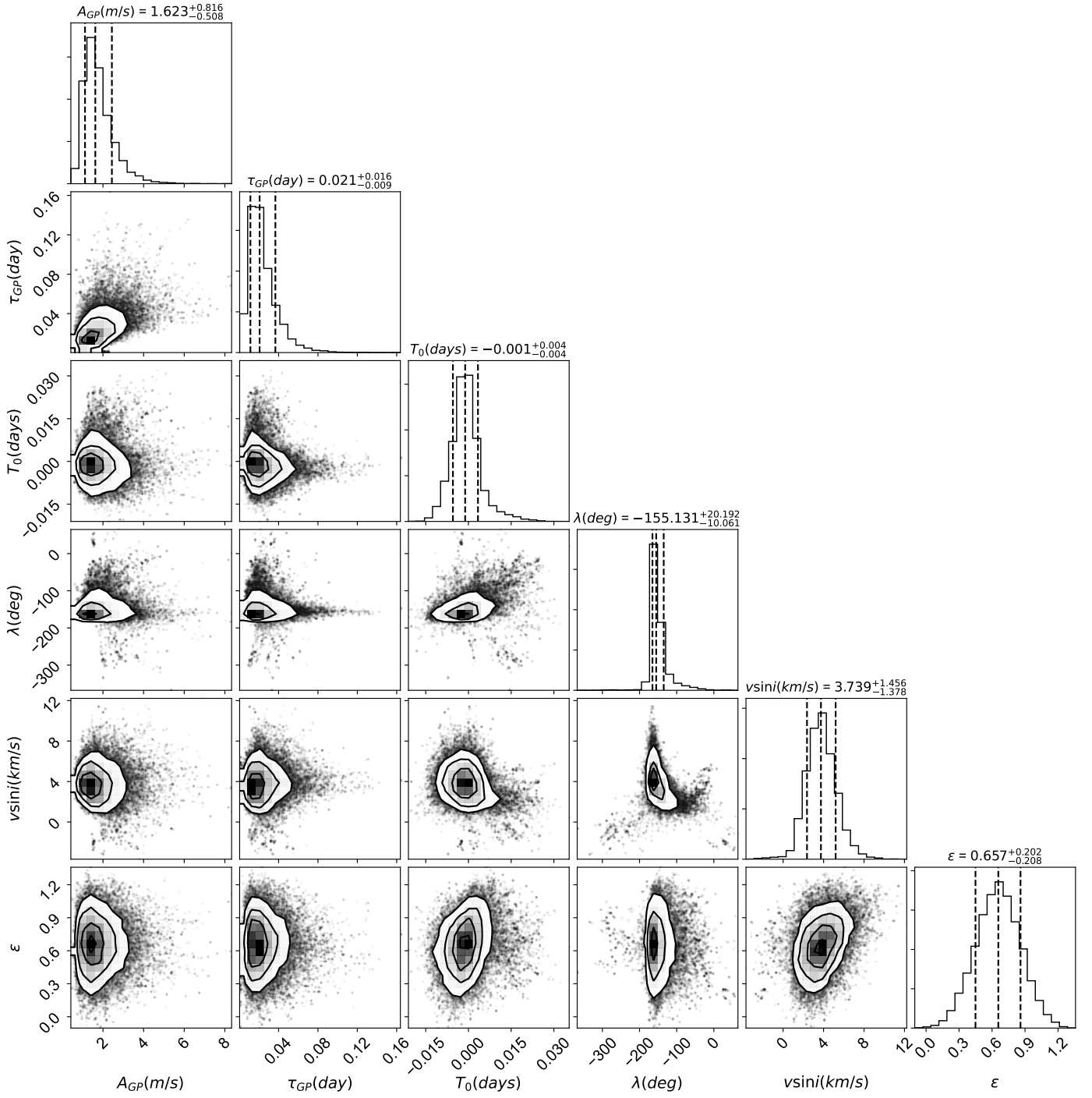
Fig. A.1. Best fit of Pyastronmy+GP
