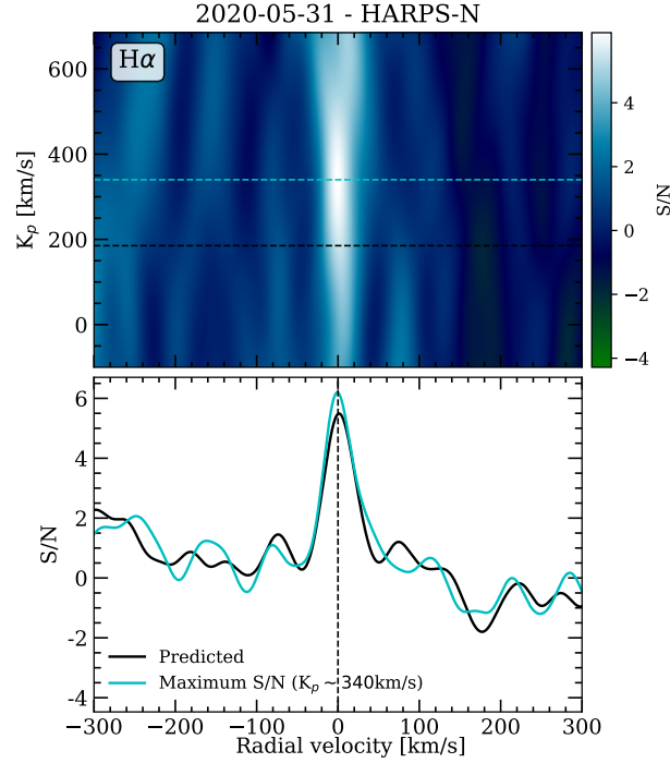
Fig. A.2. Cross-correlation results around the H \alpha line of the first night. Top panel: K_p map of the cross-correlation values. The cyan-dashed line indicates the K_p position with maximum S/N. The horizontal black dashed line shows the predicted K_p = 188.15 \text{ km s}^{-1} value, the cyan-dashed line the K_p \sim 340 \text{ km s}^{-1} at which the S/N is maximum, and the vertical black dashed line shows 0 \text{ km s}^{-1} shift. Bottom panel: cross-correlation values extracted at the maximum S/N K_p (cyan), and at the predicted K_p (black).
