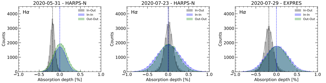
Fig. A.3. Empirical Monte Carlo (EMC) distributions in the H \alpha line for the first (left) and second (middle) nights observed with HARPS-N, and the night observed with EXPRES (right). The distributions are obtained using 20 000 iterations and measuring the absorption depth with a bandwidth of 0.75 \text{ \AA} . Each panel corresponds to the analysis of one night. In green we present the ‘out-out’ scenario, in blue the ‘in-in’, and in grey the ‘in-out’, which corresponds to the atmospheric absorption scenario. The blue-dashed vertical line marks the zero absorption level and the black-dashed line the center of the ‘in-out’ distribution.
