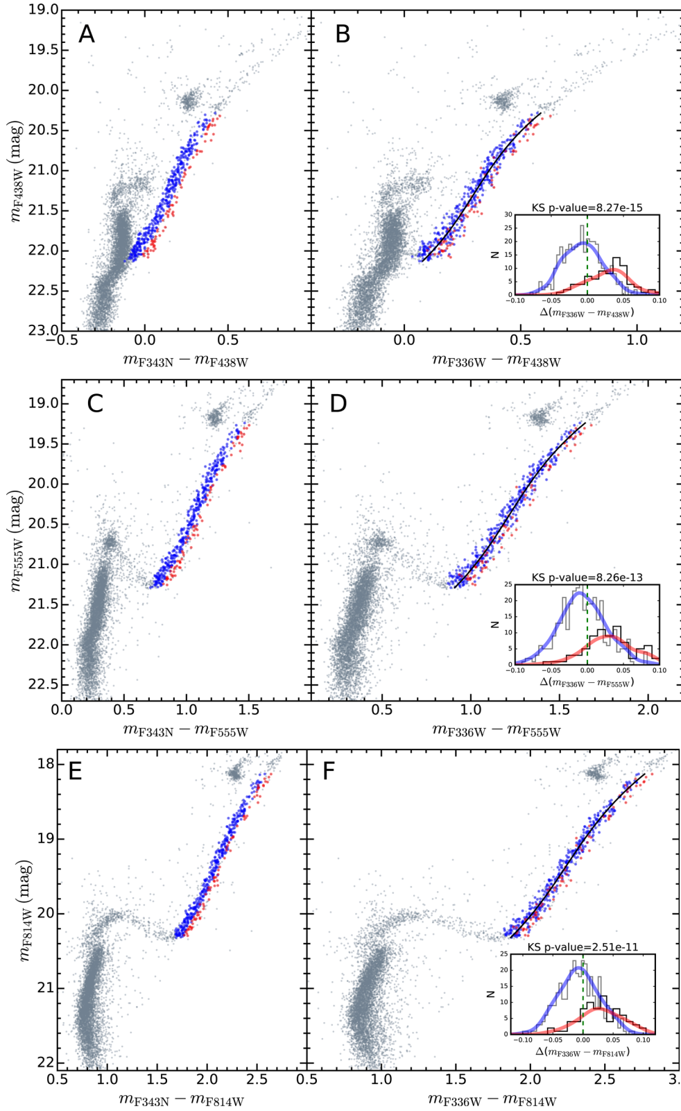
Figure 4. CMDs of NGC 1978 in U - B versus B (panel A), U - B versus B (panel B), U - V versus V (panel C), U - V versus V (panel D), U - I versus I (panel E), U - I versus I (panel F). Blue (red) filled circles mark the selected FP (SP). The black solid lines mark the defined fiducial lines. In the insets of the right-hand panels, the histograms of the distribution of the RGB FP (grey) and SP (black) stars is shown, in \Delta(U - B) (panel B), \Delta(U - V) (panel D), and \Delta(U - I) (panel F) colours. The blue (red) thick curve represents the KDE for the FP (SP) stars. The dashed green line represents the verticalized fiducial line.
