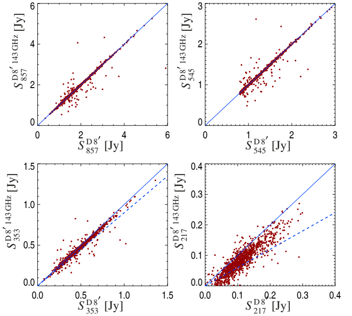
Fig. A.1. Comparison of the flux densities of the PHZ source candidates (at 8') computed on the cleaned maps obtained using the Planck 143-GHz map ( S_v^{D8'143} ) or the SMICA CMB component map ( S_v^{D8'} ) as a CMB template during the cleaning processing. The blue line provides the 1:1 reference. The dashed line gives the expected attenuation coefficients of 10% at 353 GHz and 40% at 217 GHz due to extragalactic foreground contamination of the CMB template.
