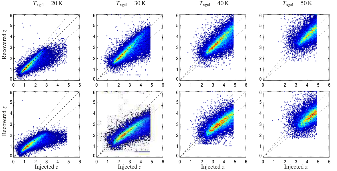
Fig. B.1. Photometric redshift recovery, for injected dust temperatures T_{\text{xgal}} = 20, 30, 40 , and 50 K (from left to right). Redshift estimates have been obtained assuming the exact dust temperature for each source, and an ideal CMB template. The 2D histogram of the recovered redshift estimates versus the injected redshifts are shown for two cases of the quality of the CMB template used for cleaning: ideal ( top ) or highly contaminated ( bottom ). The dotted lines show the \pm 20\% limits around the 1:1 relation (dashed line).
