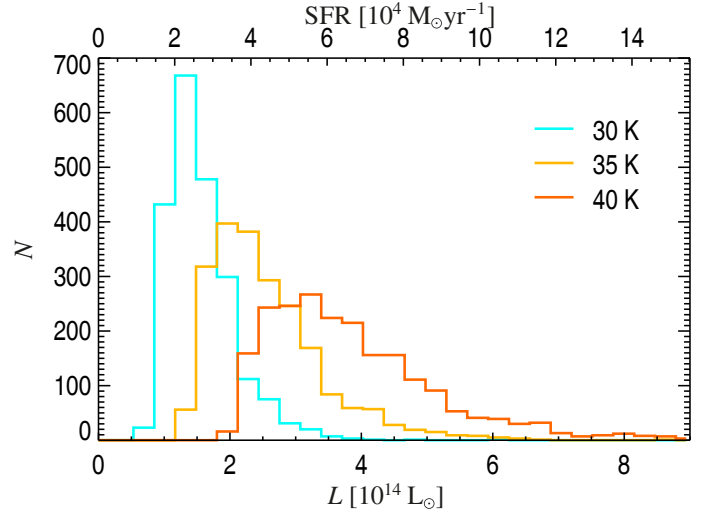
Fig. 17. Distribution of the FIR bolometric luminosity and SFR for three assumptions of the extragalactic dust temperature, T_{\text{xgal}} = 30, 35 , and 40 K.
