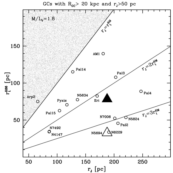
Figure 10. Jacobi radii versus tidal radii of the best-fitting K66 model for Galactic GCs more distant than 20 kpc from the Galactic Centre and having Jacobi radius larger than 50 pc (the latter selection has been introduced to make the plot as easy to read as possible; NGC 2419 is not included in the plot since it has a Jacobi radius much larger than all the other clusters, r_J = 604.4 pc). Lines at fixed r_J/r_t^{KM} ratio are also plotted for reference. NGC 5694 is plotted as an empty triangle when the K66 tidal radius is adopted, and as a filled triangle when the radius of the outermost point of our SB profile is adopted instead. The shaded area correspond to the region of overfilling clusters.
