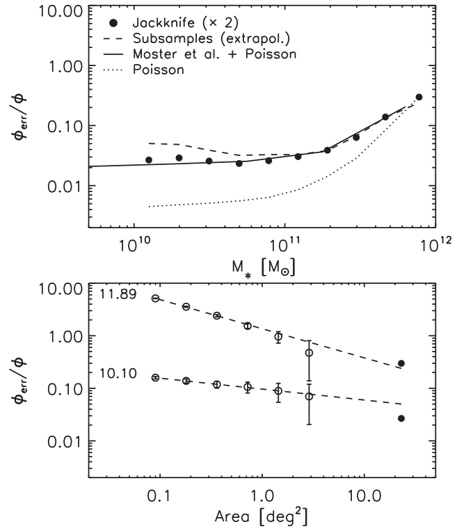
Figure 3. Stellar mass function statistical errors as function of stellar mass (top) and area (bottom). In the top panel, we show the jackknife estimator based on 64 subregions and multiplied by a factor of 2, compared to the theoretical cosmic variance plus Poisson error derived from the Moster et al. (2011) GETCV code (the Poisson error only is shown as the dotted line). The bottom panel shows an alternative internal estimate based on the standard deviation of subsamples as a function of their size, in two mass bins ( \log M_*/M_\odot = 10.10 and 11.89 ), extrapolated to the size of the full survey (dashed lines in both panels). As in the top panel, the black dots are the jackknife estimates, for which the cosmic variance part has been multiplied by 2.
