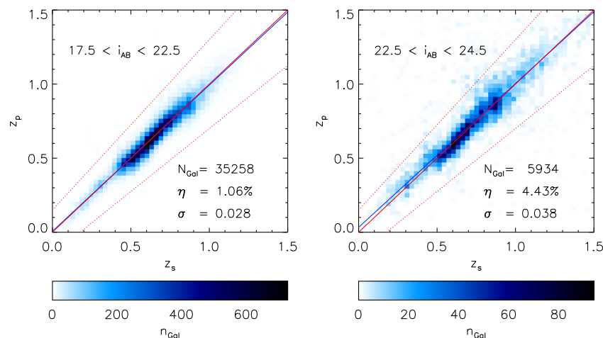
Figure 2. Photometric redshifts measured with ugrizK (left) or ugrizJHK (right) photometry versus VIPERS and VVDS spectroscopic redshifts. Left: 17.5 < i < 22.5 , where the sample is dominated by galaxies between 0.5 < z < 1.2 due to the VIPERS selection. Right: 22.5 < i < 24.5 , from the VVDS Deep and Ultra-Deep surveys. The limits for the outliers are shown as red dotted lines.
