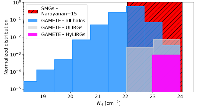
Figure 6. The blue histogram shows the distribution of N_H predicted for the overall population of galaxies in our model, while the grey and magenta histograms show the distribution of N_H predicted for the ULIRG and HyLIRG progenitors of the z \sim 6 quasar host galaxies, respectively. The N_H distribution for ULIRGs is consistent with the distribution of N_H predicted for SMGs by the cosmological hydrodynamical simulation by Narayanan et al. (2015) (red hatched region).
