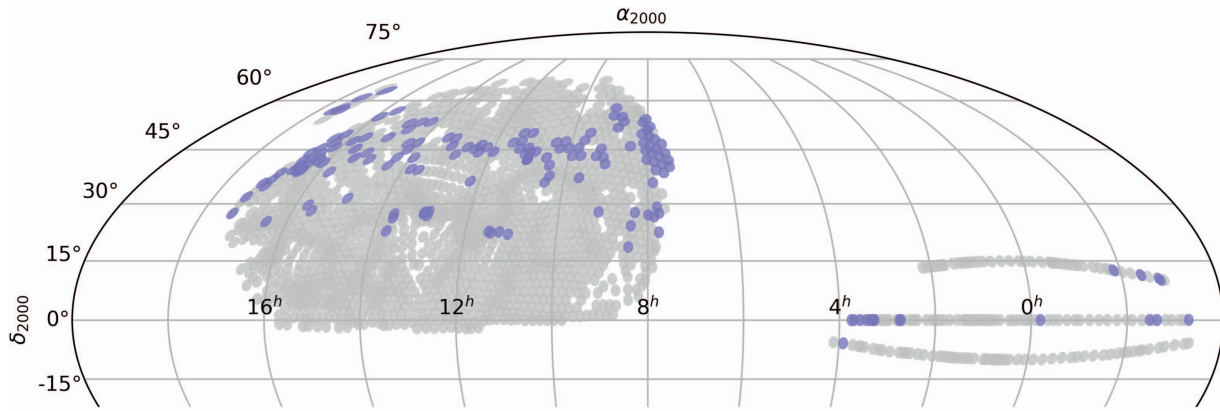
Figure 5. Sky distribution (Mollweide equatorial projection for decl. > -20^\circ ) of possible MaNGA plates (in light gray). Because MaNGA targets are selected from a sample with SDSS-I photometry and redshifts, this footprint corresponds to the Data Release 7 imaging data (Abazajian et al. 2009). Each plate contains 17 MaNGA targets, and around 30% of all possible plates will be observed in the full six-year survey. The dark purple indicates plates with data released as part of DR14.
