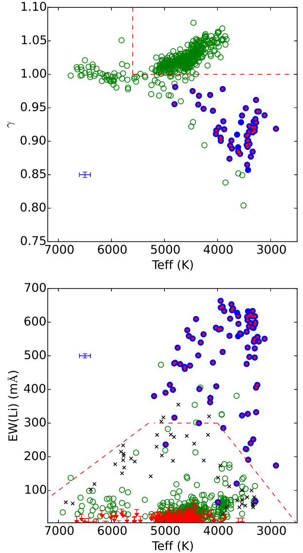
Fig. 3. Gravity index \gamma and EW(Li) as a function of the stellar effective temperature ( upper and lower panel , respectively). The index \gamma and the EW(Li) measured from the GES spectra are indicated with circles: the empty green circles are the non-members, the filled blue circles are the cluster members, and the red dots represent the members already known from previous studies. Upper limits are indicated by red downward arrows. Median error bars are shown on the left for both panels. The black crosses in the bottom panel are the EW(Li) measured for stars in the 30–50 Myr open cluster IC 2602 by Randich et al. (1997, 2001). In both panels, the dashed red lines indicate the threshold used to separate members and non-members. In the bottom panel, a few stars that are above the dashed red line are reported as non-members because they have been excluded according to the criterion based on the gravity index, and other stars that are below this line are classified as members because they are strong accretors, as discussed in Sect. 3.
