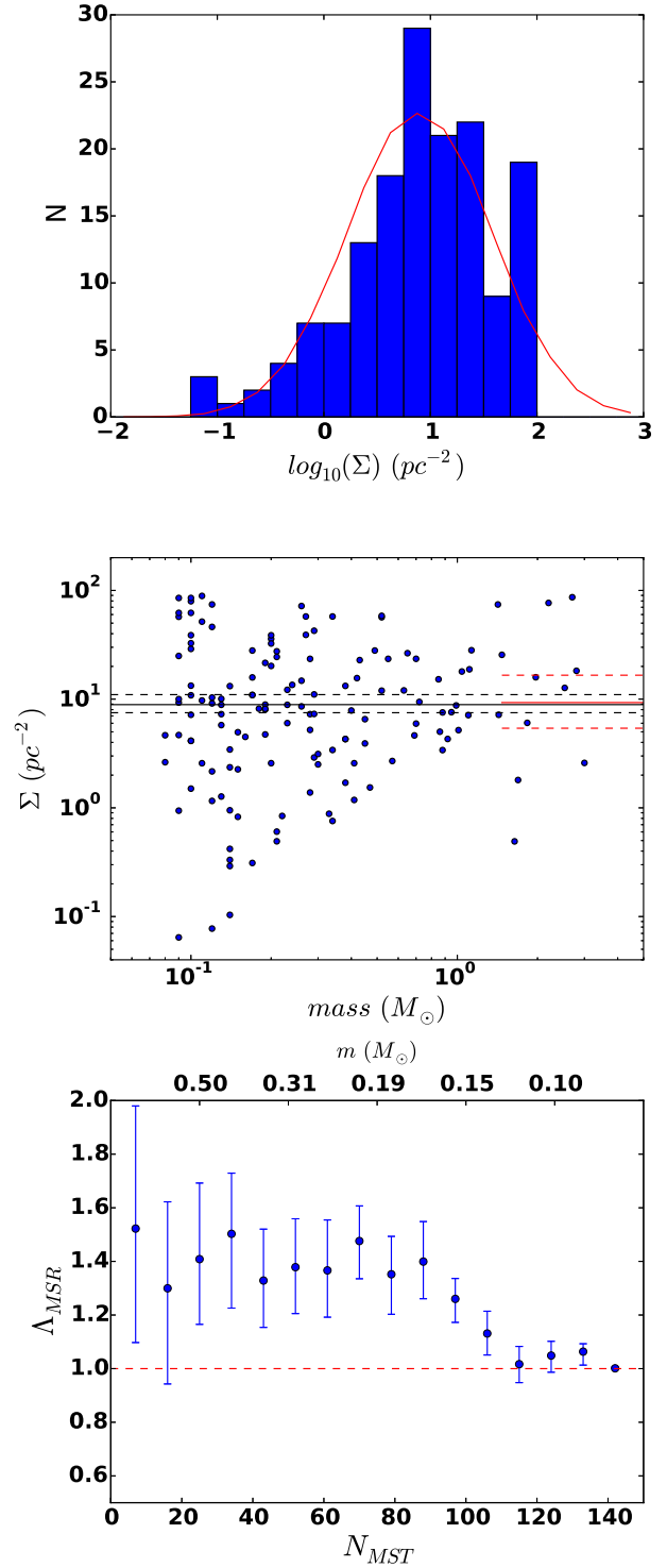
Fig. 8. Top: distribution of the surface density \Sigma and the best-fit model with a lognormal function (continuous red line). Middle: stellar density as defined in Eq. (3) as a function of the star mass. The black and red lines indicate the median density of the whole stellar sample and the ten most massive stars, respectively. The continuous lines represent the best value, while the dashed lines represent their error bars. Bottom: evolution of the mass segregation ratio, \Lambda_{\text{MSR}} , for the N_{\text{MST}} most massive stars. The top x-axis indicates the lowest mass star m_L within N_{\text{MST}} and the dashed line corresponds to \Lambda_{\text{MSR}} = 1 , i.e., no mass segregation.
