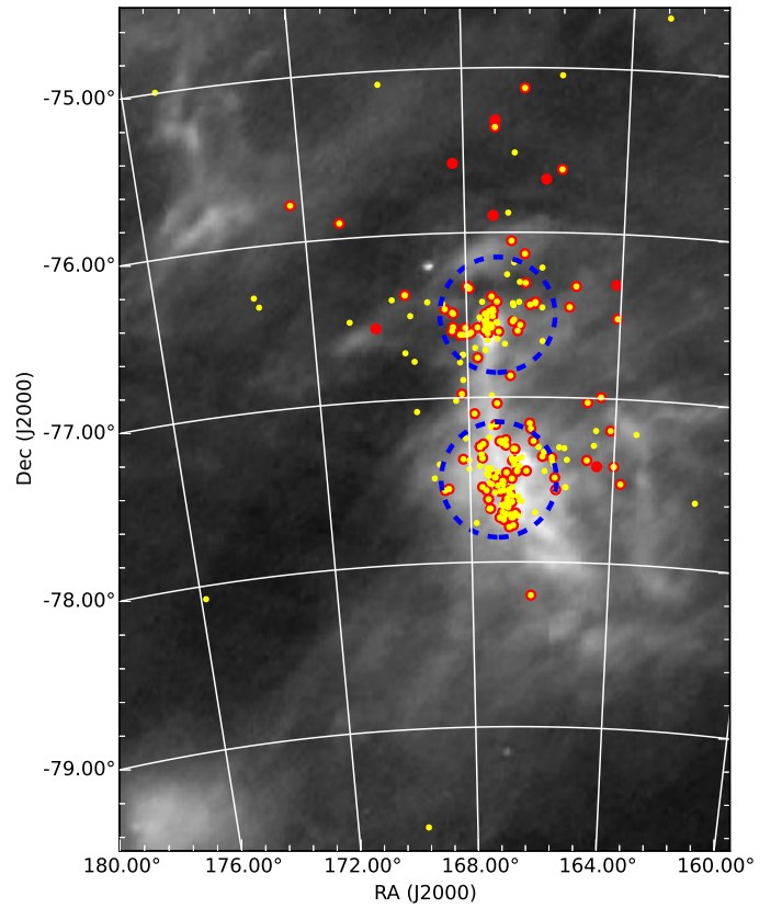
Fig. 2. Far infrared (140 \mu m) map of the region around the young cluster Cha I from the AKARI all-sky survey ( Doi et al. 2015 ). Yellow dots indicate the positions of all the known members from the literature, while the bigger red dots indicate the positions of all the members selected by the GES observations according to the criteria discussed in Sect. 3. The dashed blue circles (centers RA1 = 167.2°, Dec1 = -76.5°, RA2 = 167.2°, Dec2 = -77.5°, and radius 0.35°) delimit the north and south subclusters (see Sects. 4.2 and 5.3).
