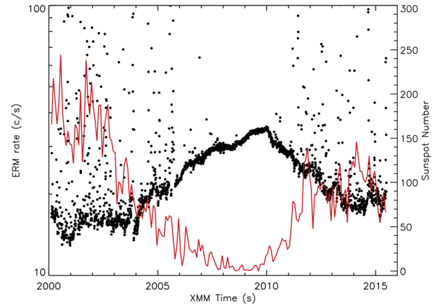
Figure 8. The median count rate of the ERM HES0 in each XMM-Newton orbit is shown as a function of time. The y-axis range has been clipped to a value of 100 counts s -1 and error bars have been omitted for clarity of the plot. The number of Sun spots is over-plotted with a red line.
